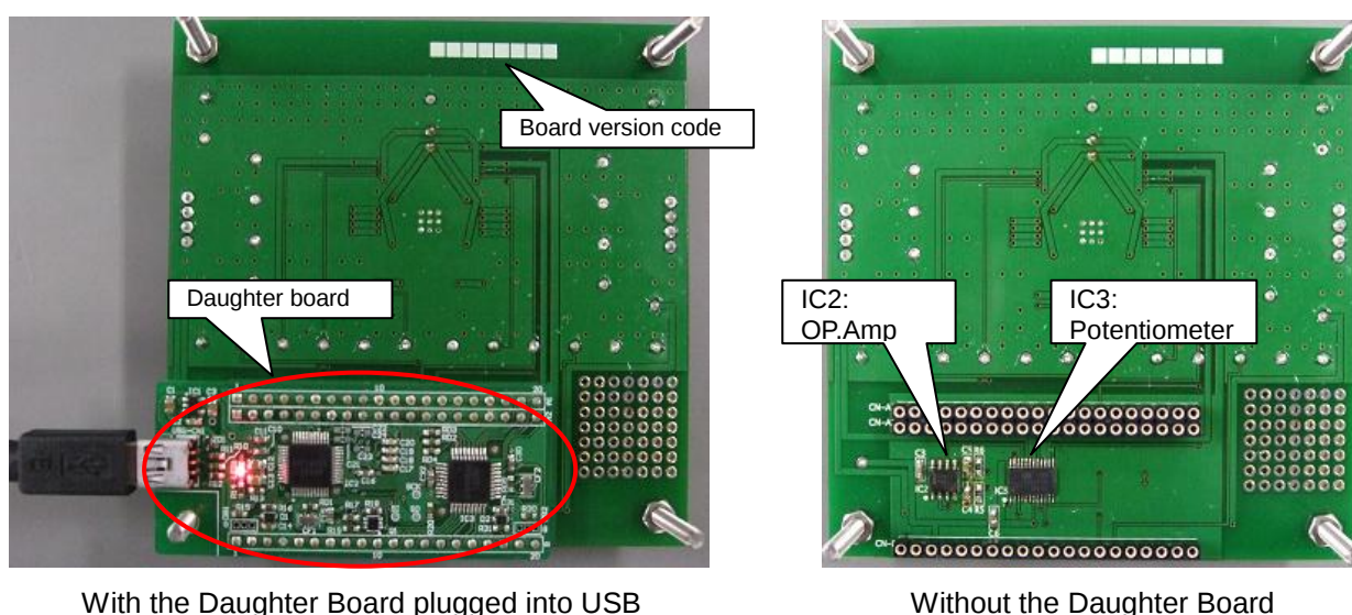
Figure 2. Bottom view of the Evaluation Board
