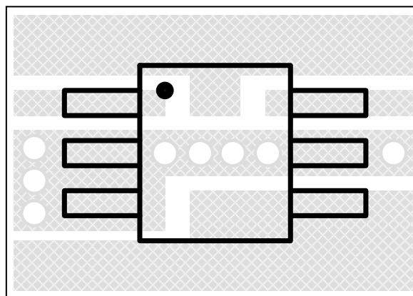
Figure 36 Board Via Layout For Thermal Dissipation
