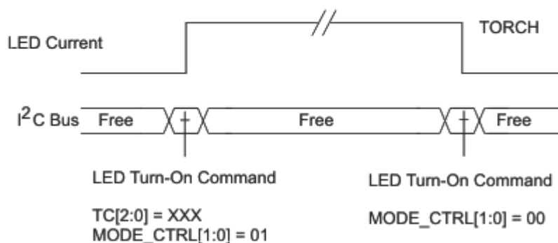
Figure 18. Torch Mode Operation
