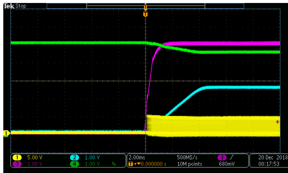
Figure 5. TPS50601ASPEVM Start-Up Relative to V_{IN}
