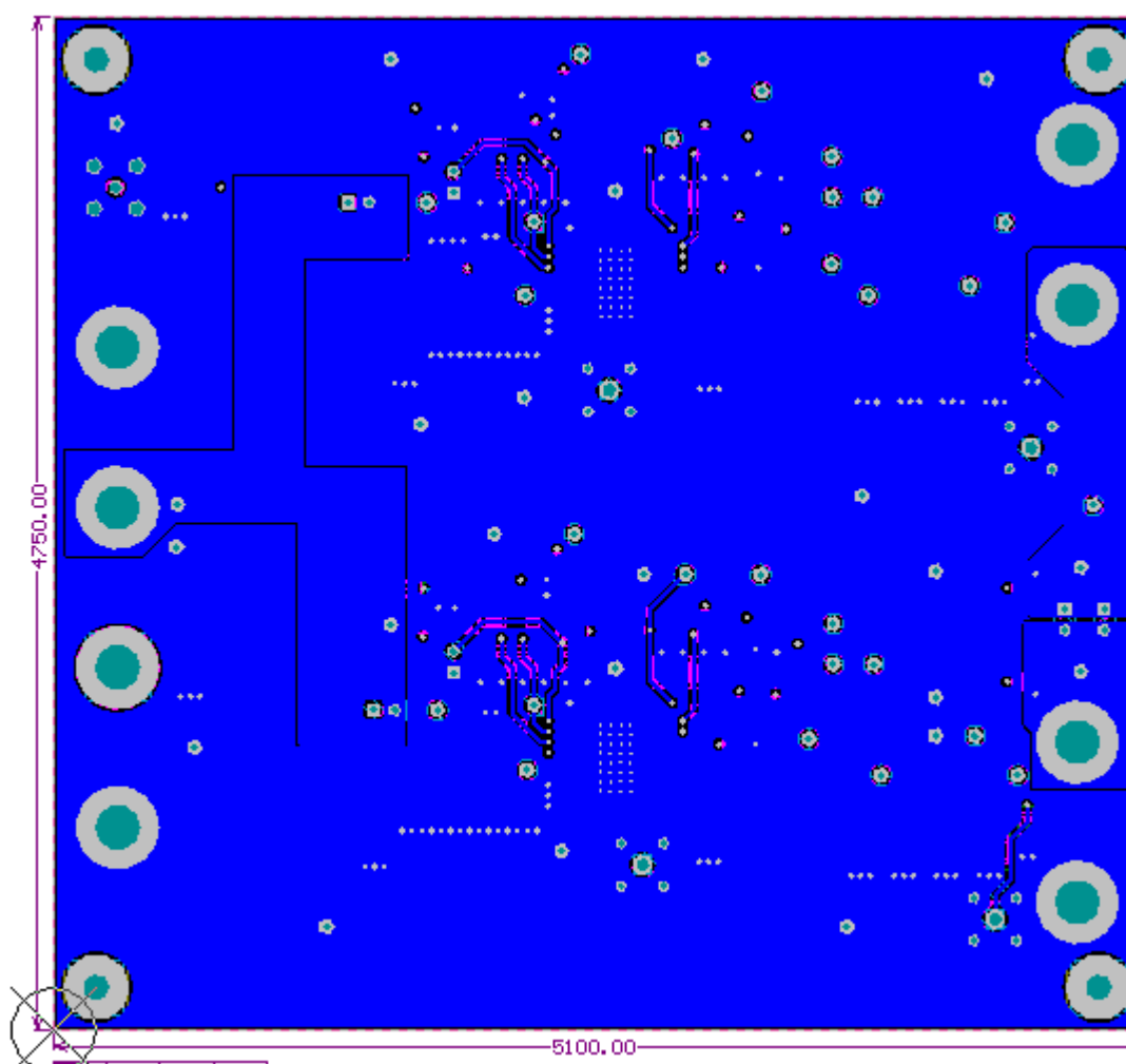
Figure 11. TPS50601ASPEVM Bottom-Side Layer 4
