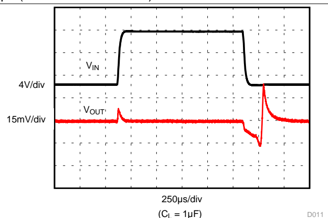
Figure 14. Line Transient
