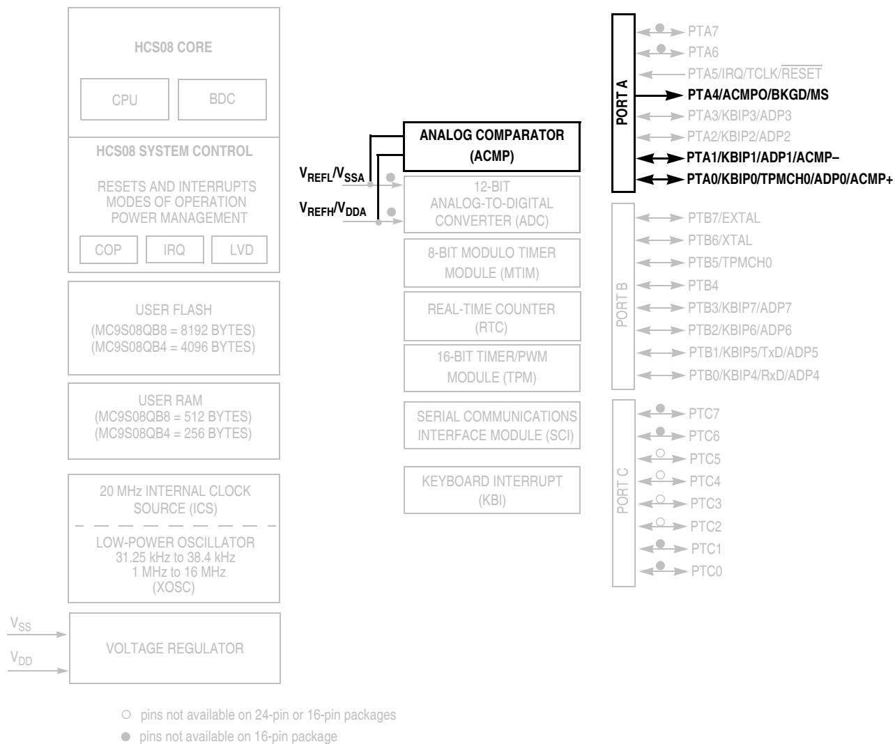
Figure 9-1. MC9S08QB8 Series Block Diagram Highlighting ACMP Block and Pins
