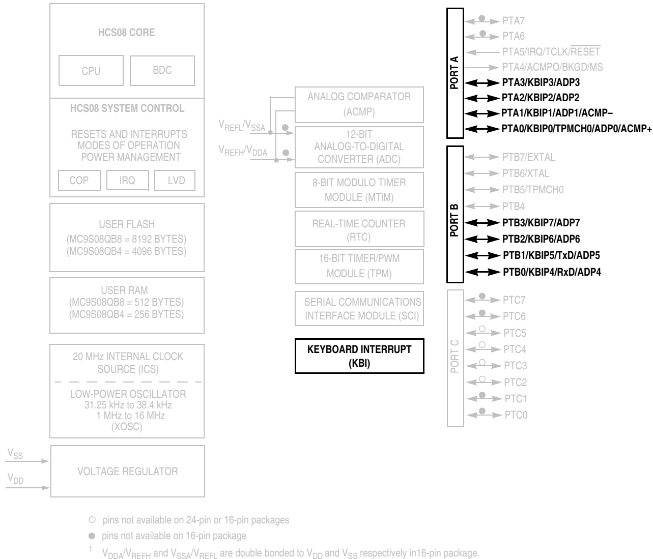
Figure 7-1. MC9S08QB8 Series Block Diagram Highlighting KBI Block and Pins
