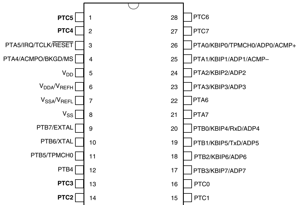
Figure 2-1. MC9S08QB8 Series in 28-Pin SOIC Package
