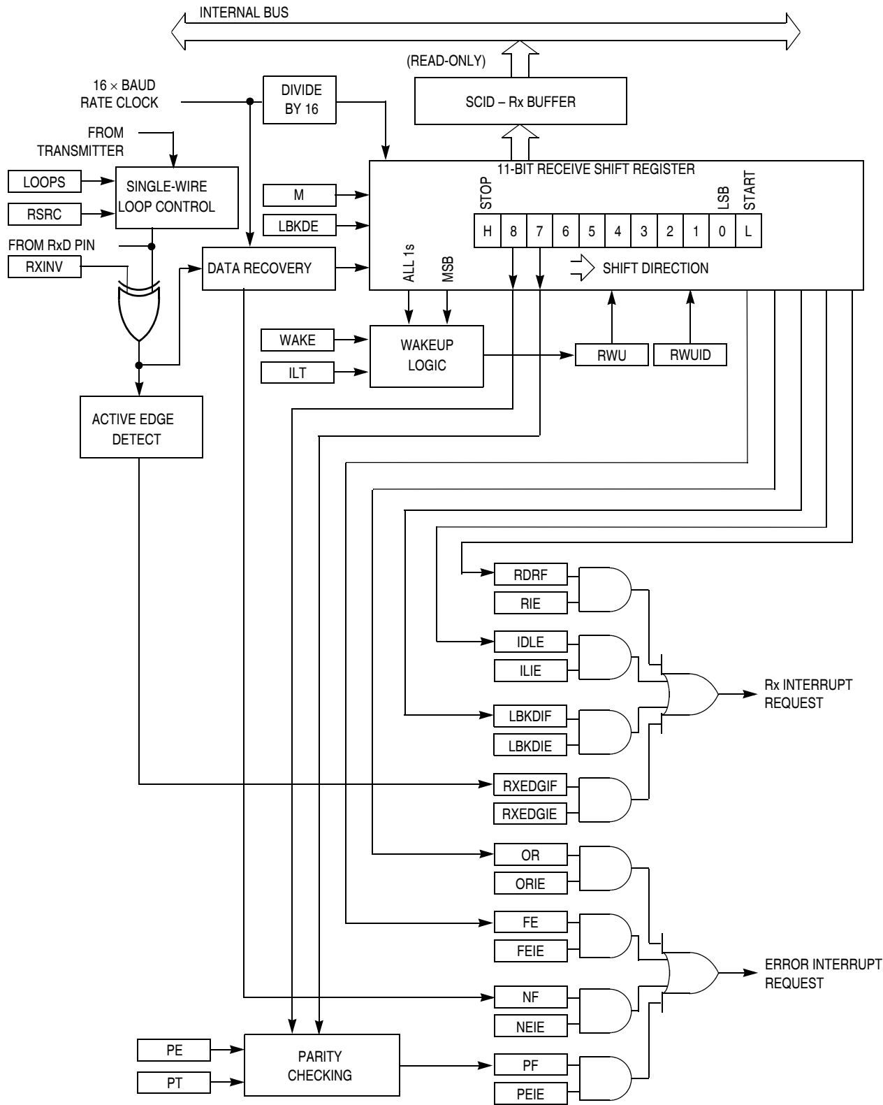
Figure 14-4. SCI Receiver Block Diagram
