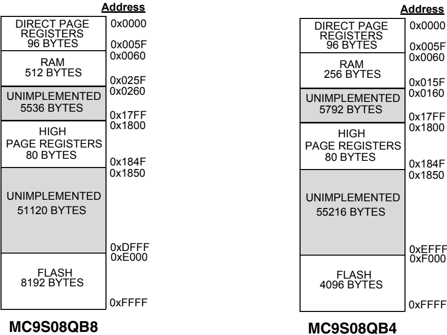
Figure 4-1. MC9S08QB8 Series Memory Maps
