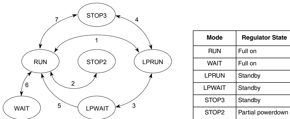
Figure 3-1. Allowable Power Mode Transitions for the MC9S08QB8 Series
