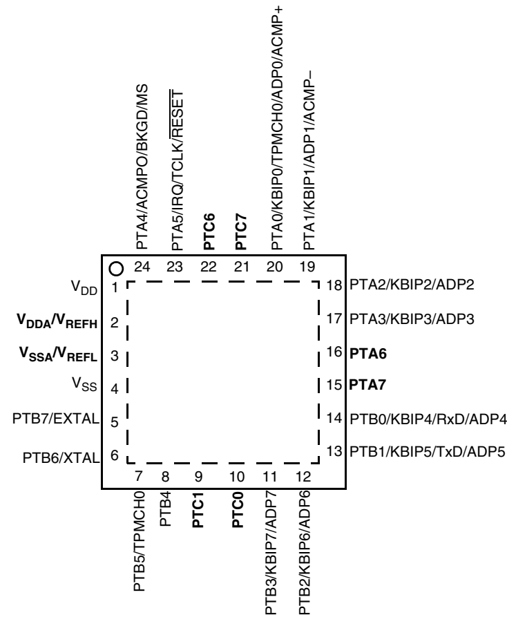
Figure 2-2. MC9S08QB8 Series in 24-Pin QFN Packages
