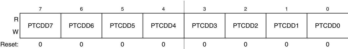
Figure 6-13. Port C Data Direction Register (PTCDD)
