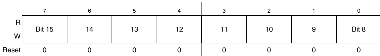
Figure 15-13. TPM Channel Value Register High (TPMCnVH)
