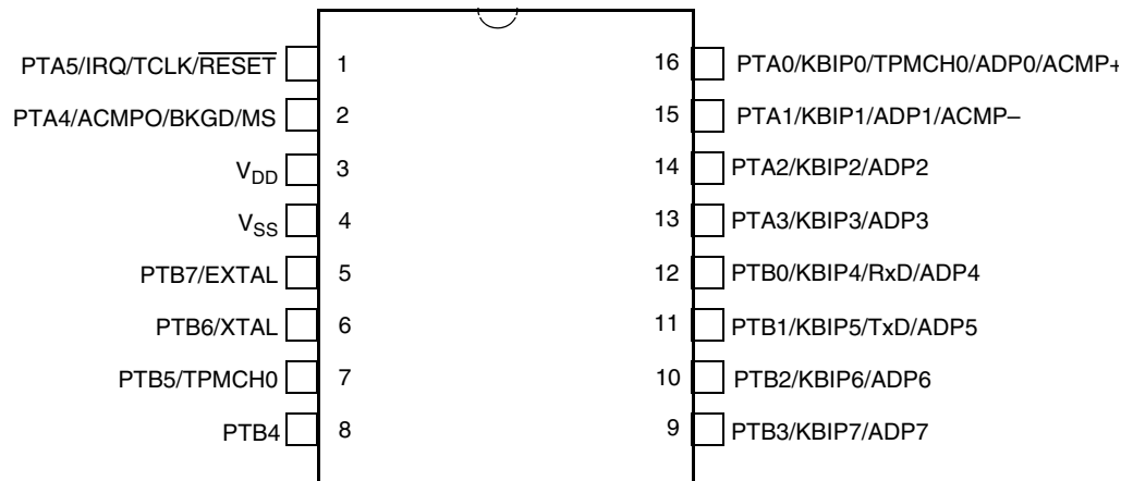
Figure 2-3. MC9S08QB8 Series in 16-Pin TSSOP Packages
