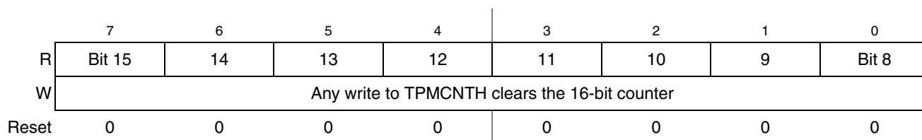
Figure 15-8. TPM Counter Register High (TPMCNTH)
