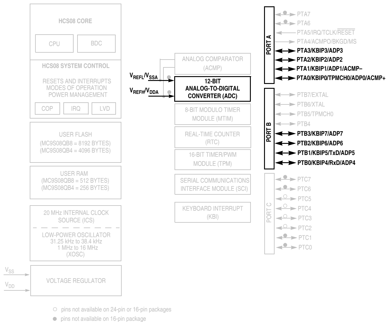
Figure 10-1. MC9S08QB8 Series Block Diagram Highlighting ADC Block and Pins
