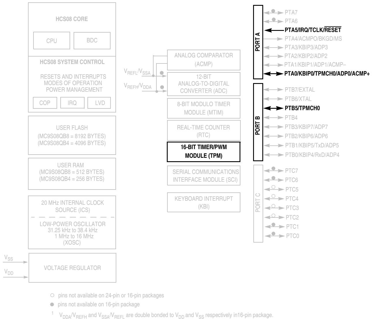
Figure 15-1. MC9S08QB8 Series Block Diagram Highlighting TPM Block and Pins
