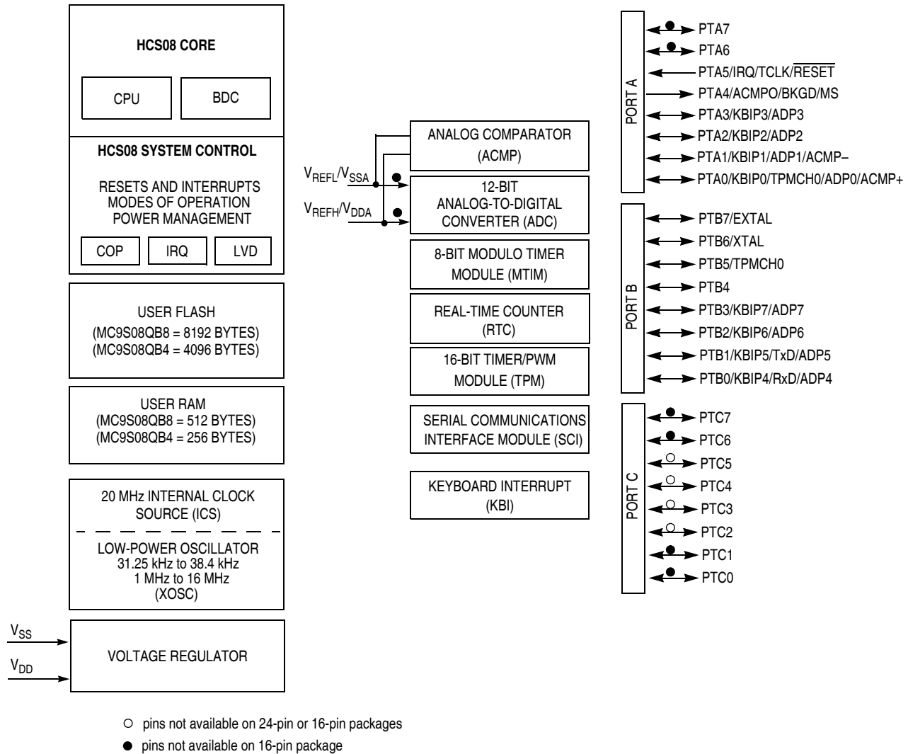
Figure 1-1. MC9S08QB8 Series Block Diagram
