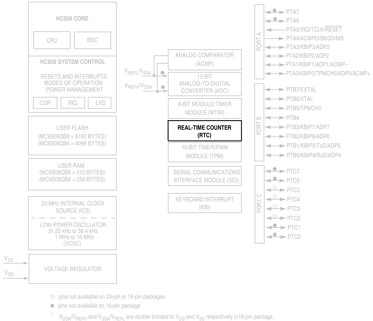
Figure 13-1. MC9S08QB8 Block Diagram Highlighting RTC Block
