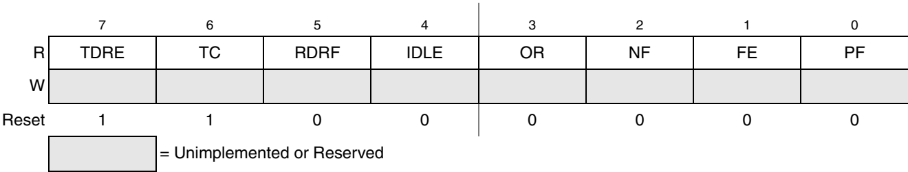
Figure 14-9. SCI Status Register 1 (SCIS1)
