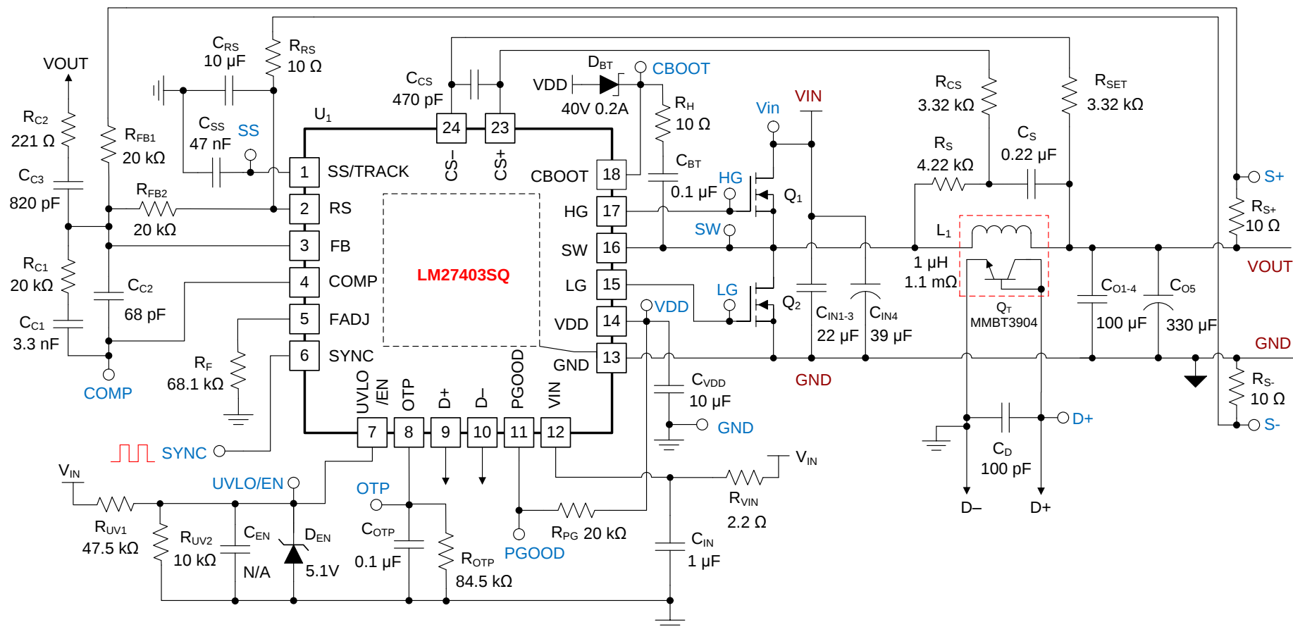
Figure 1. Circuit Diagram
