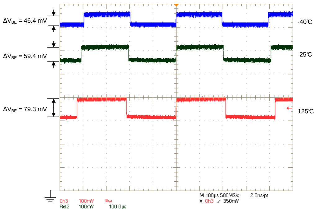
Figure 24. D+ Voltage ( \Delta V_{BE} ) at -40°C, 25°C, 125°C Operating Temperatures
