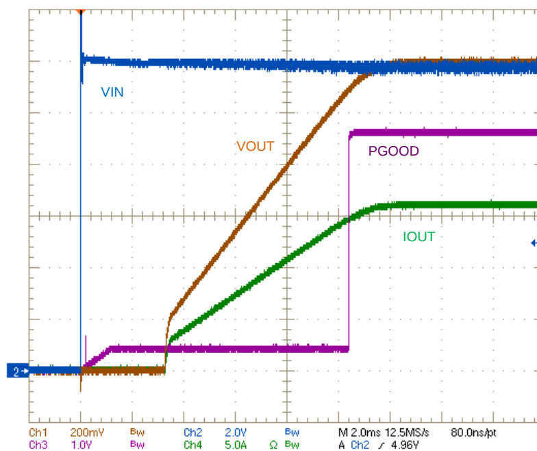
Figure 14. Startup with VIN Stepped to 12 V; V_{OUT} = 1.2 V, 70-mΩ Load
