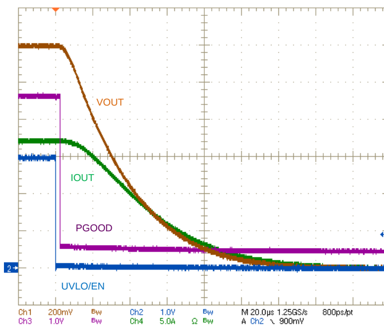
Figure 19. Shutdown with UVLO/EN Pulled To GND; V_{IN} = 12\text{ V} , V_{OUT} = 1.2\text{ V} , 70-m \Omega Load
