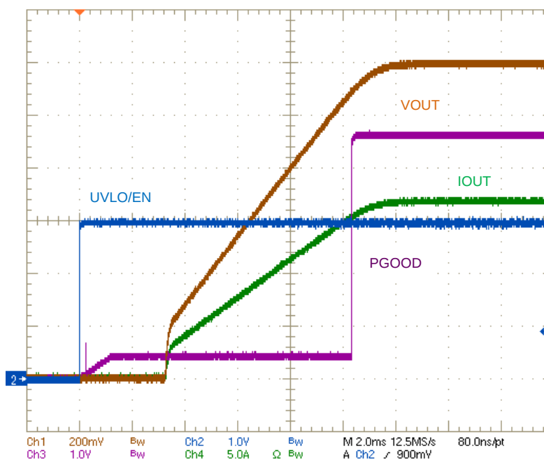
Figure 18. Startup with UVLO/EN Stepped to 3 V; V_{IN} = 12\text{ V} , V_{OUT} = 1.2\text{ V} , 70-m \Omega Load
