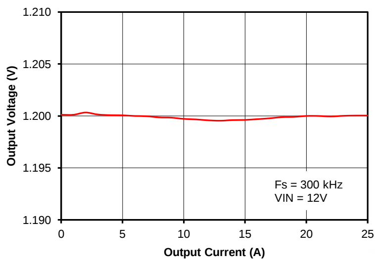
Figure 6. Load Regulation
