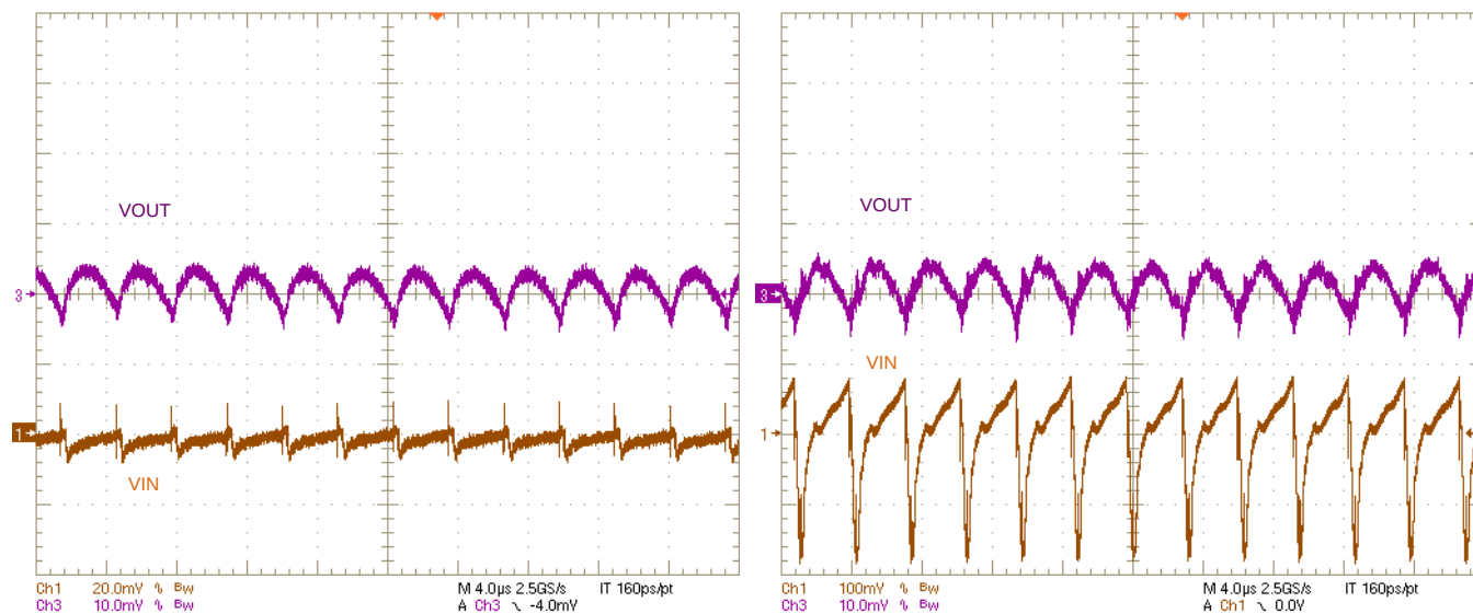
Figure 12. Input and Output Voltage Ripple; V_{IN} = 12\text{ V} , V_{OUT} = 1.2\text{ V} , I_{OUT} = 0\text{ A} and 25\text{ A}
