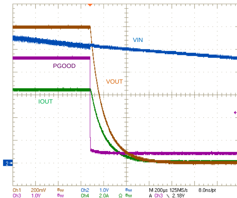
Figure 15. Shutdown After VIN Disconnected; V_{IN} = 12 V, V_{OUT} = 1.2 V, 200-mΩ Load
