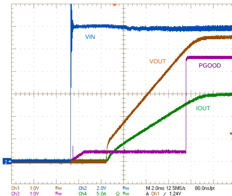
Figure 17. Startup with V_{IN} Stepped to 12 V; V_{OUT} = 5.5 V, 340-mΩ Load
