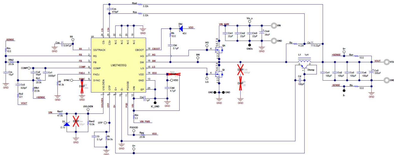
Figure 25. Schematic
