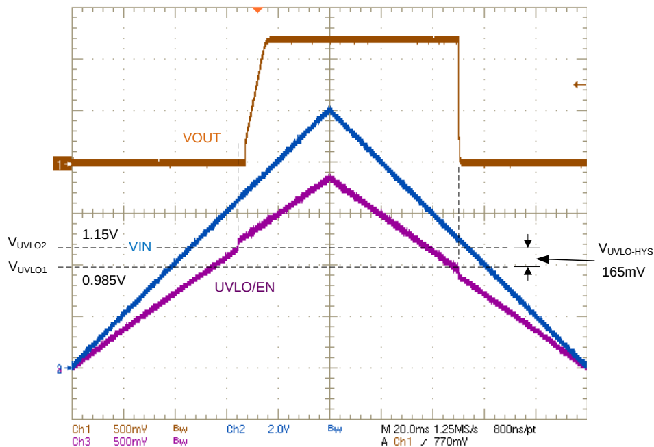
Figure 16. Startup with V_{IN} Ramping Slowly 0 V – 8 V – 0 V; V_{OUT} = 1.2 V, 200-mΩ Load
