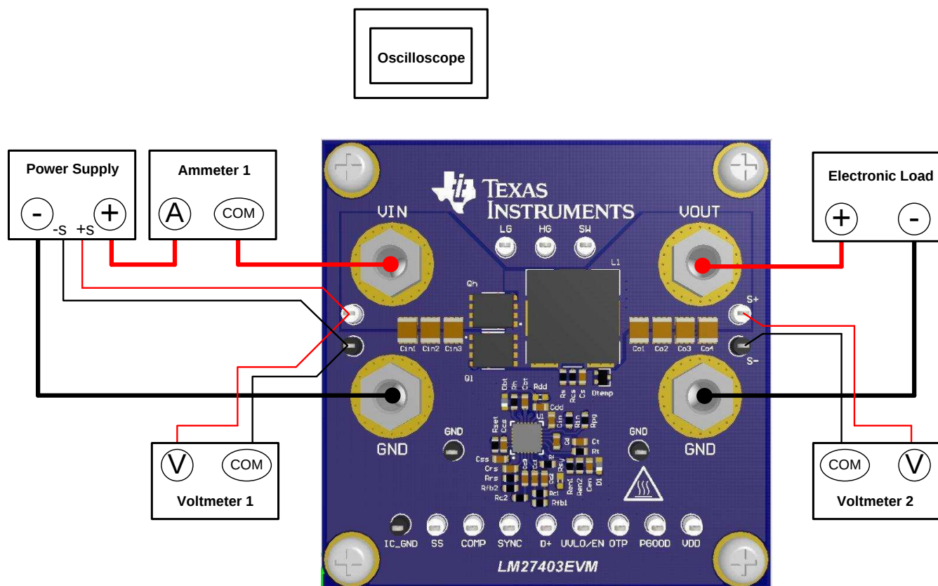
Figure 3. Connection Diagram
