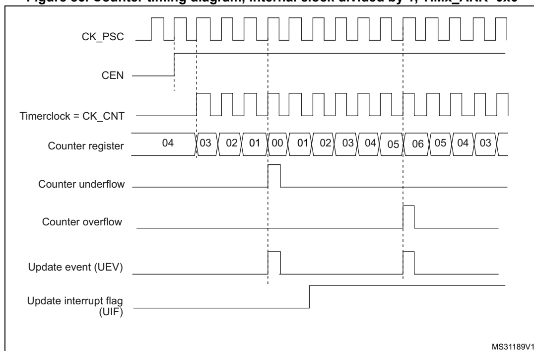
Figure 86. Counter timing diagram, internal clock divided by 1, TIMx_ARR=0x6
