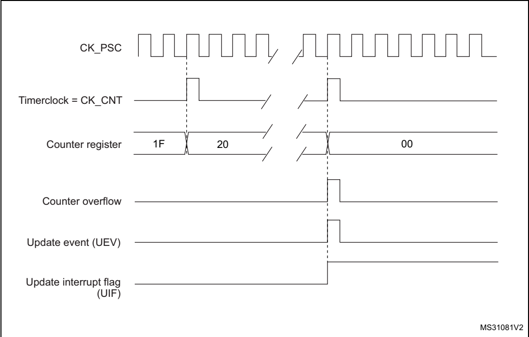
Figure 78. Counter timing diagram, internal clock divided by N
