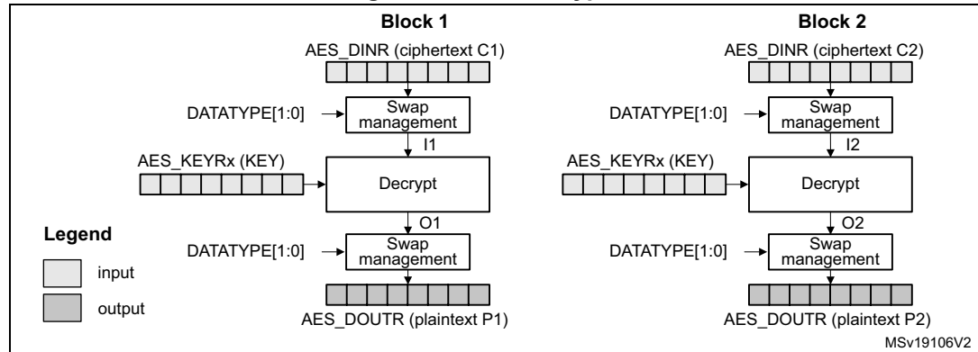
Figure 60. ECB decryption
