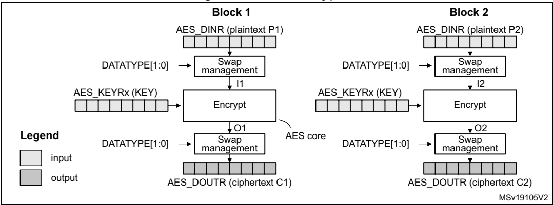
Figure 59. ECB encryption
