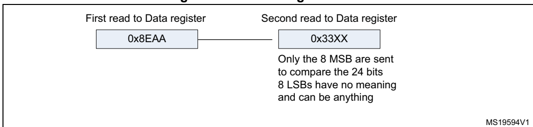
Figure 264. Receiving 0x8EAA33
