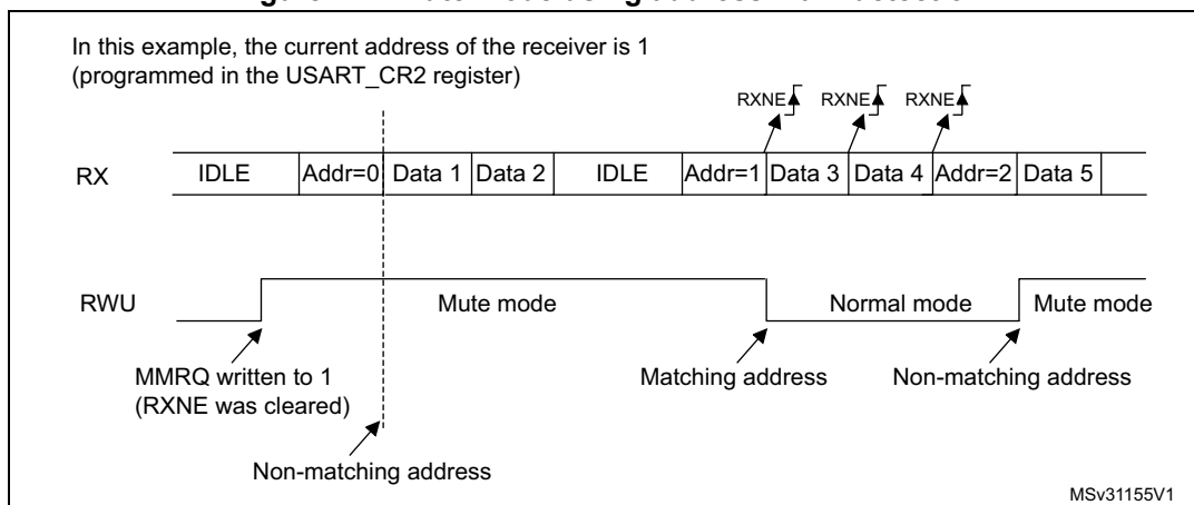
Figure 217. Mute mode using address mark detection
