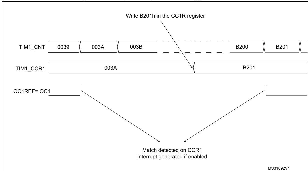
Figure 101. Output compare mode, toggle on OC1.
