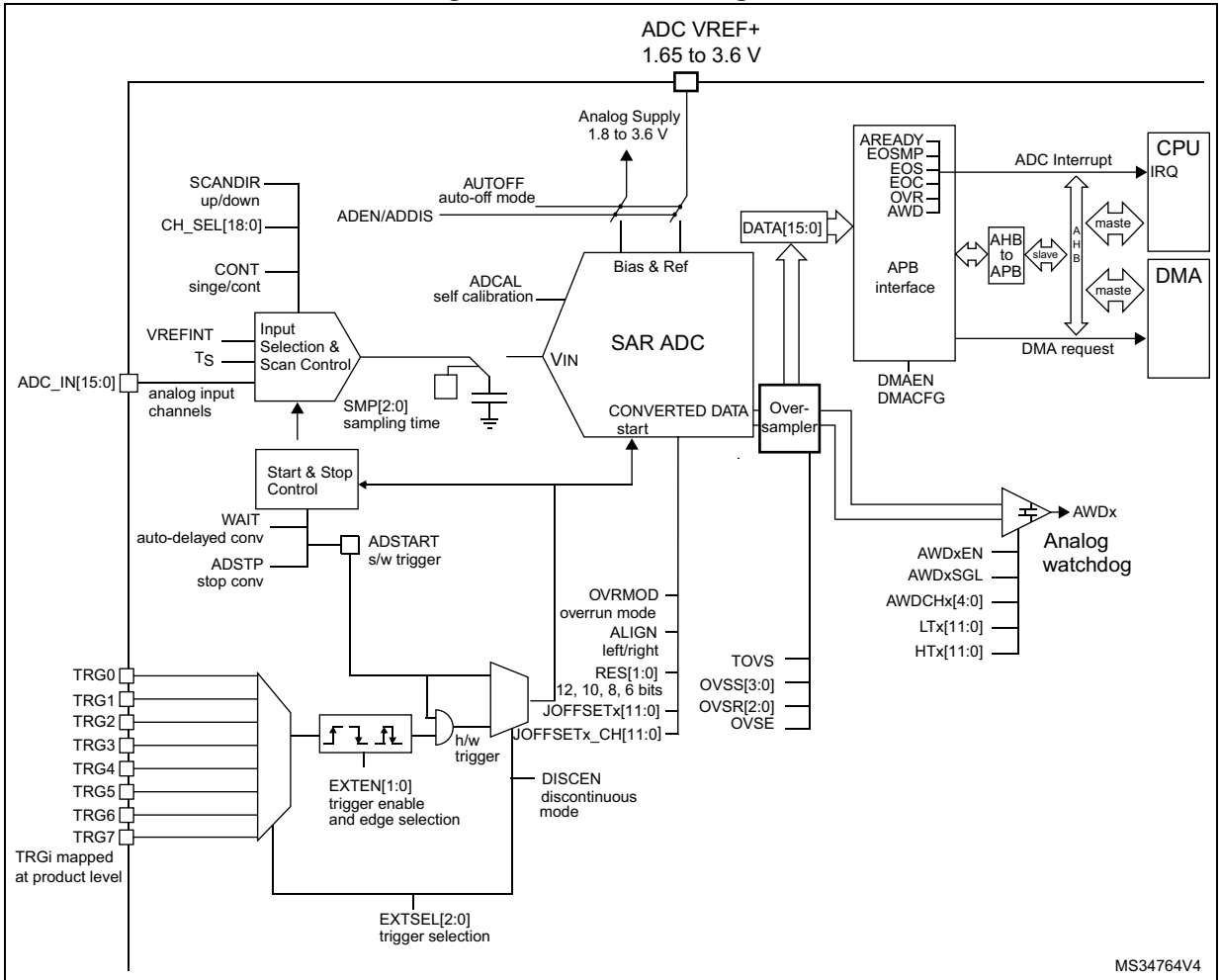
Figure 29. ADC block diagram
