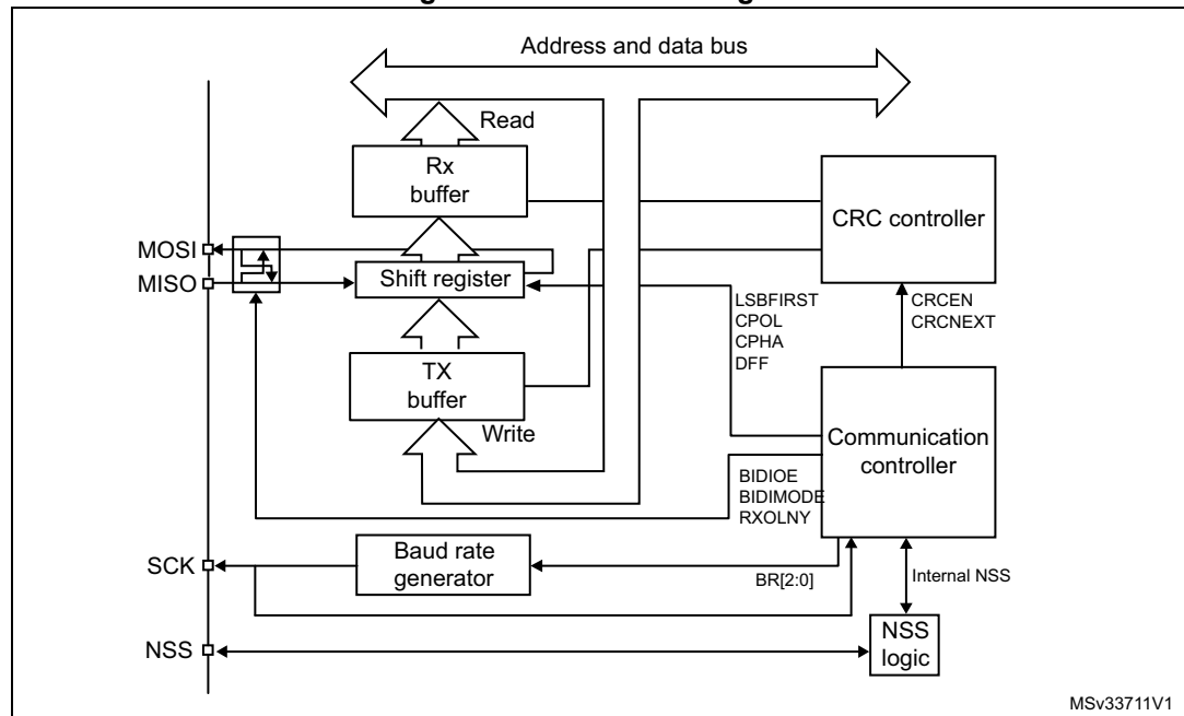
Figure 246. SPI block diagram
