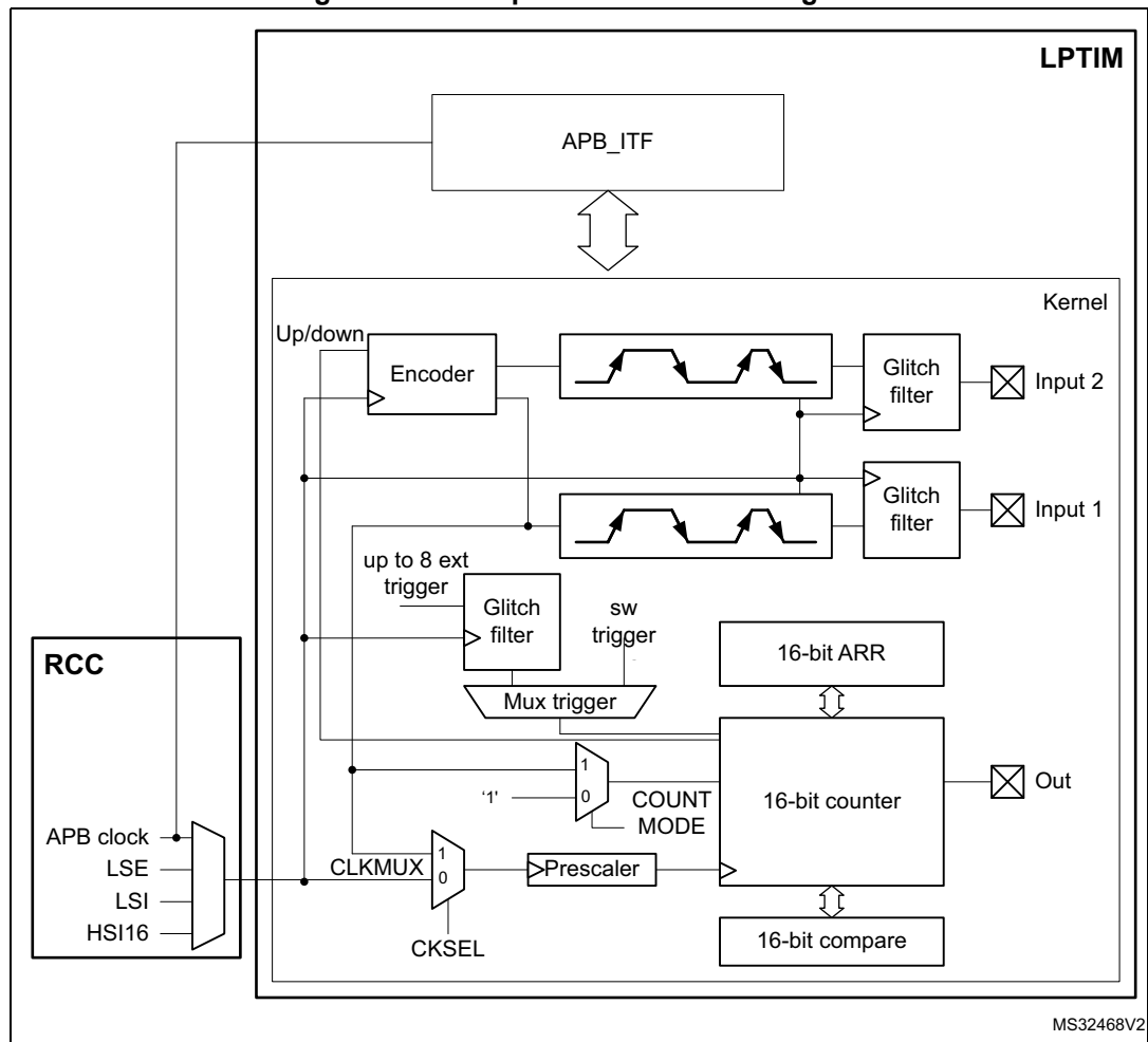
Figure 166. Low-power timer block diagram
