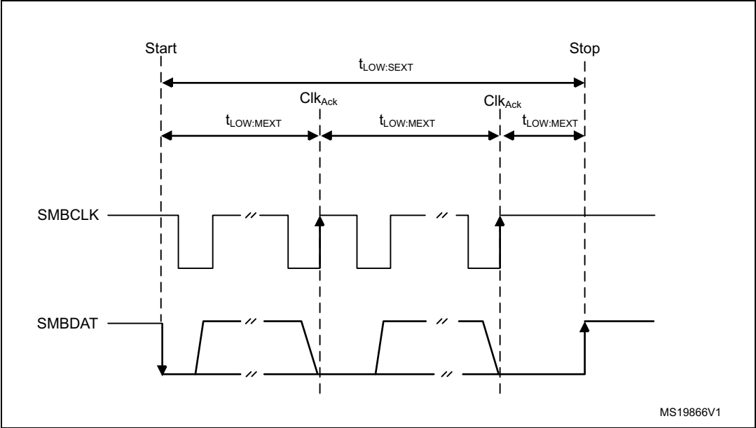
Figure 201. Timeout intervals for t_{\text{LOW:SEXT}} , t_{\text{LOW:MEXT}}
