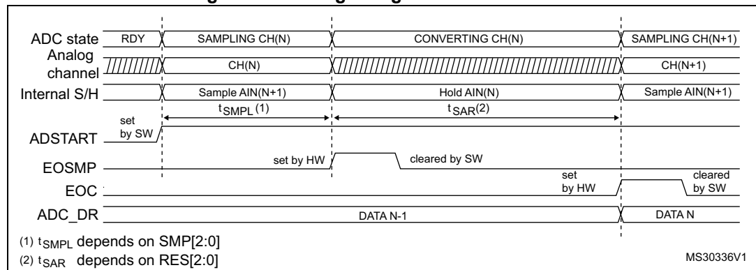
Figure 34. Analog to digital conversion time
