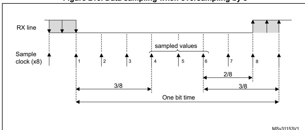
Figure 215. Data sampling when oversampling by 8
