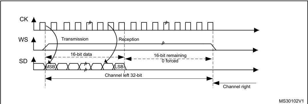
Figure 269. MSB justified 16-bit extended to 32-bit packet frame with CPOL = 0
