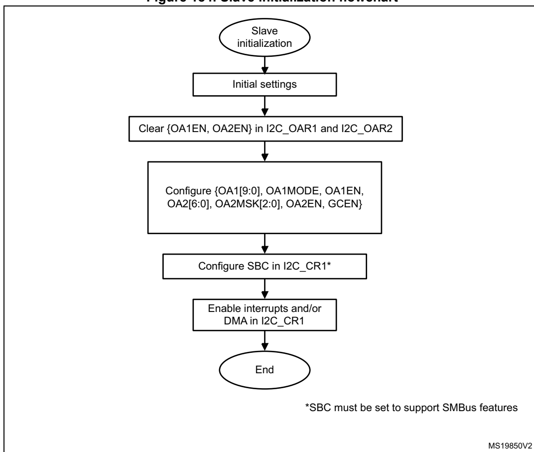
Figure 184. Slave initialization flowchart
