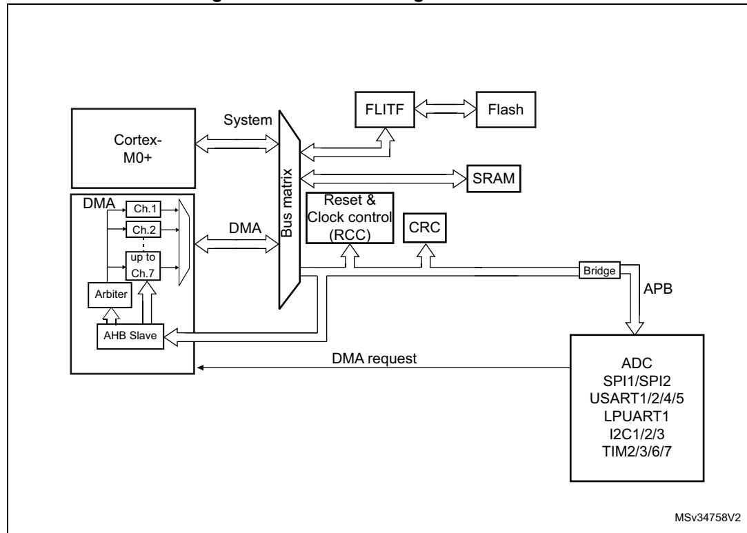
Figure 25. DMA block diagram
