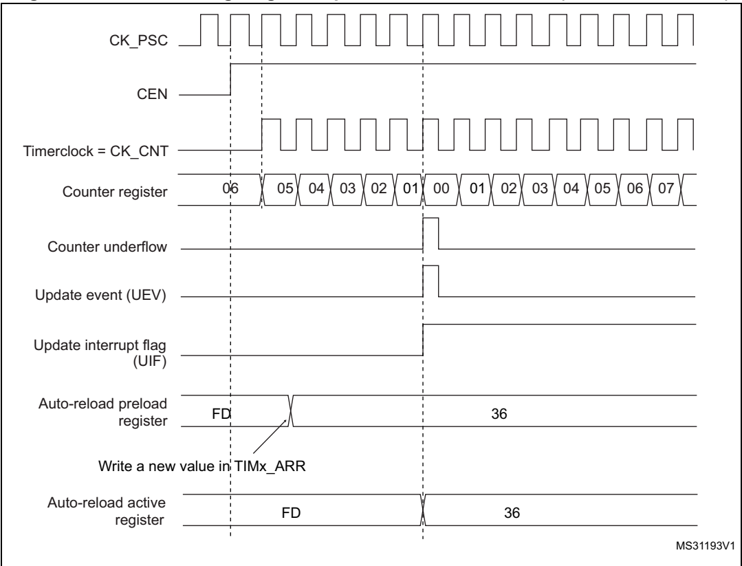
Figure 90. Counter timing diagram, Update event with ARPE=1 (counter underflow)
