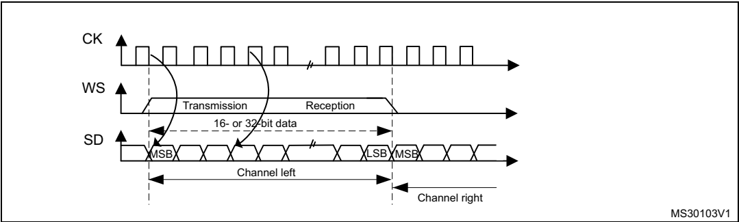
Figure 270. LSB justified 16-bit or 32-bit full-accuracy with CPOL = 0
