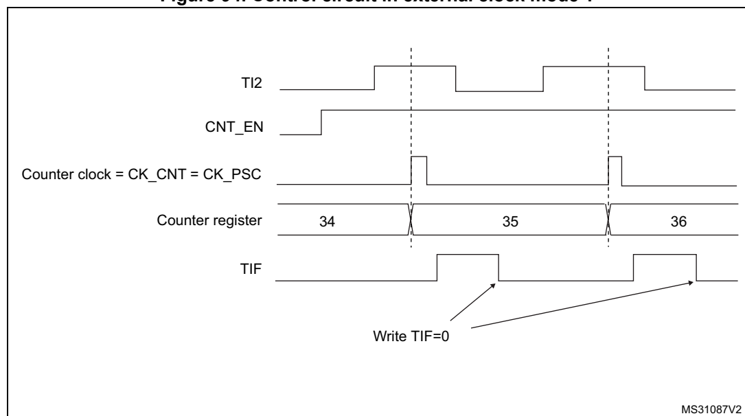
Figure 94. Control circuit in external clock mode 1
