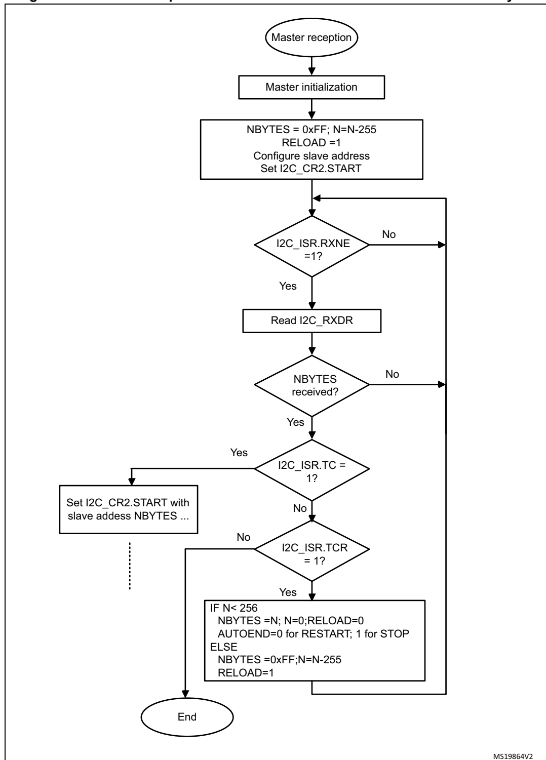
Figure 199. Transfer sequence flowchart for I2C master receiver for N &gt; 255 bytes
