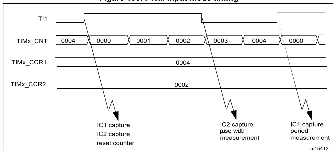
Figure 100. PWM input mode timing
