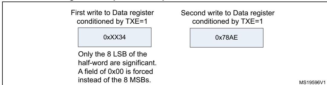
Figure 272. Operations required to transmit 0x3478AE
