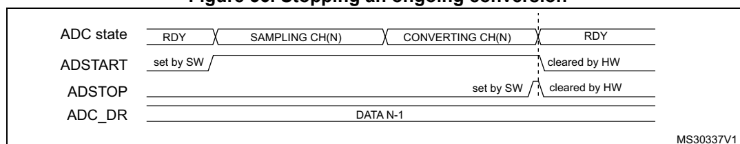
Figure 36. Stopping an ongoing conversion
