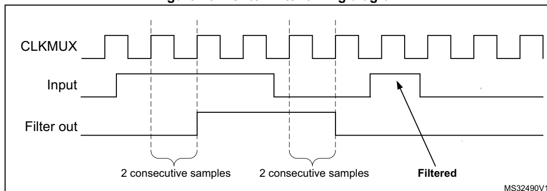
Figure 167. Glitch filter timing diagram
