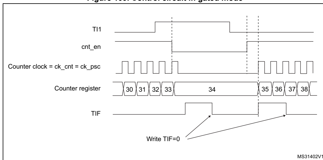
Figure 109. Control circuit in gated mode
