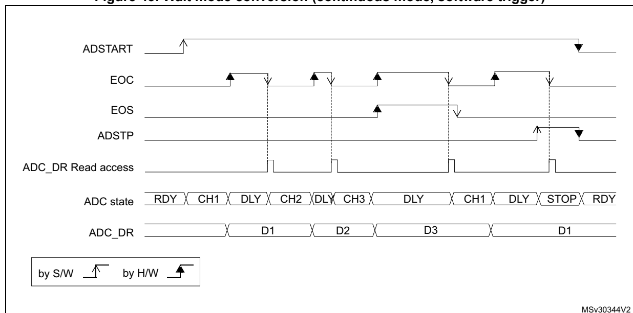
Figure 43. Wait mode conversion (continuous mode, software trigger)
