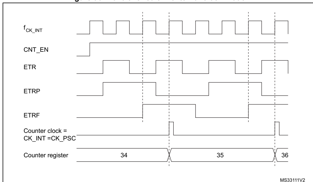
Figure 96. Control circuit in external clock mode 2
