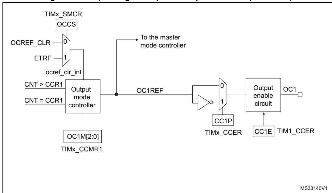
Figure 99. Output stage of capture/compare channel (channel 1)
