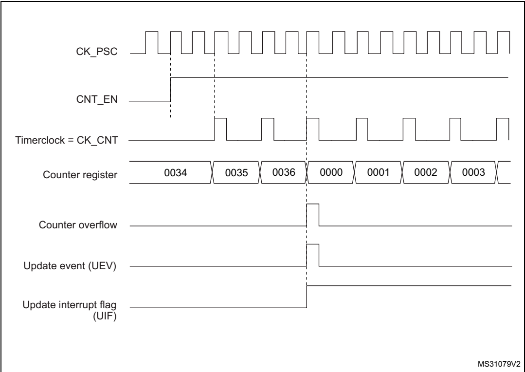
Figure 76. Counter timing diagram, internal clock divided by 2
