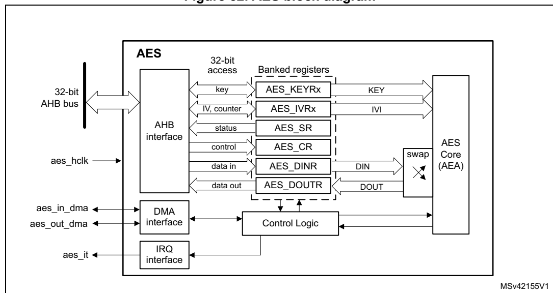
Figure 52. AES block diagram
