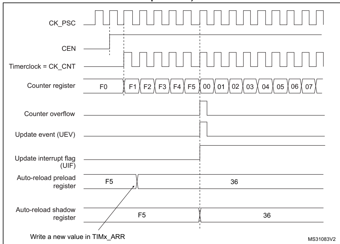
Figure 126. Counter timing diagram, update event when ARPE=1 (TIMx_ARR preloaded)
