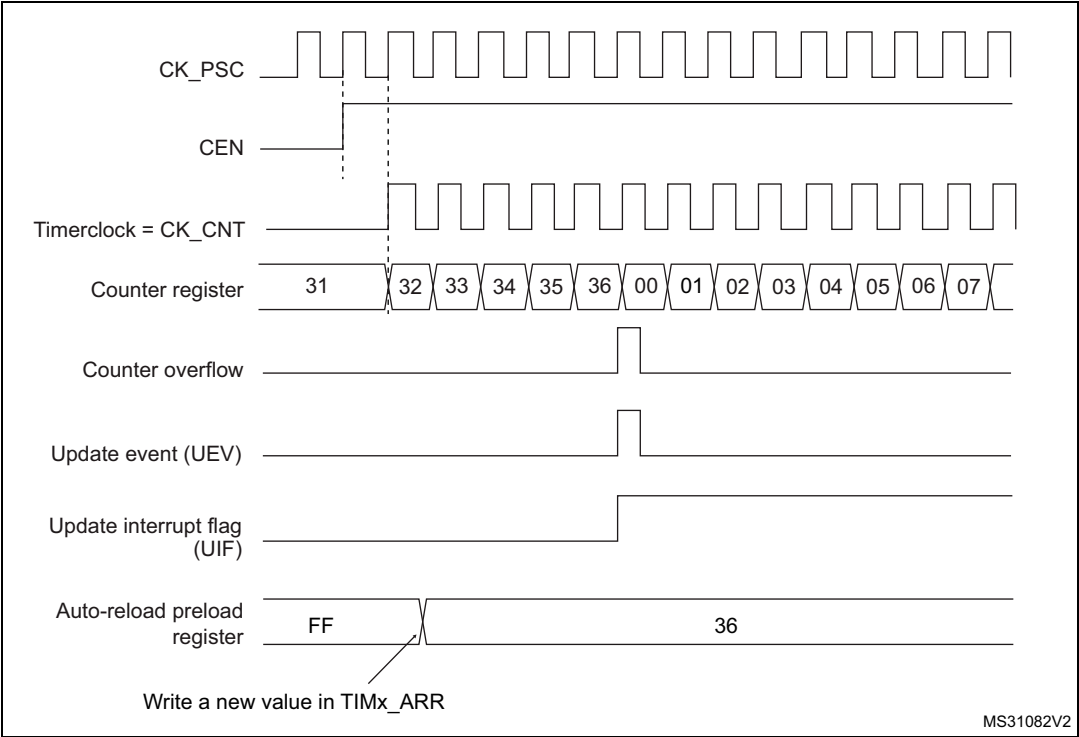
Figure 79. Counter timing diagram, Update event when ARPE=0 (TIMx_ARR not preloaded)
