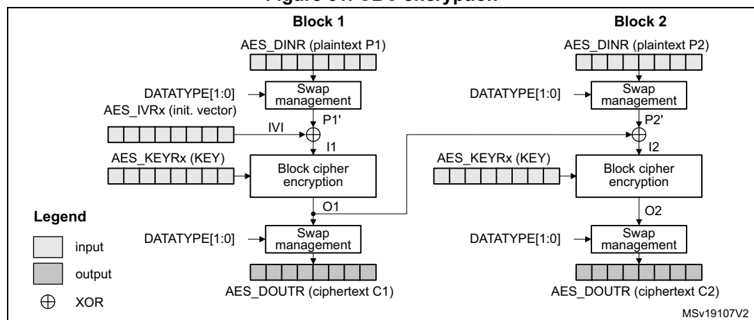
Figure 61. CBC encryption
