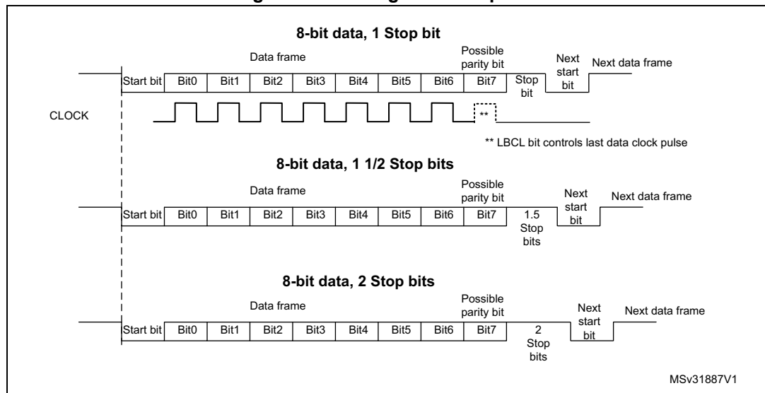
Figure 211. Configurable stop bits
