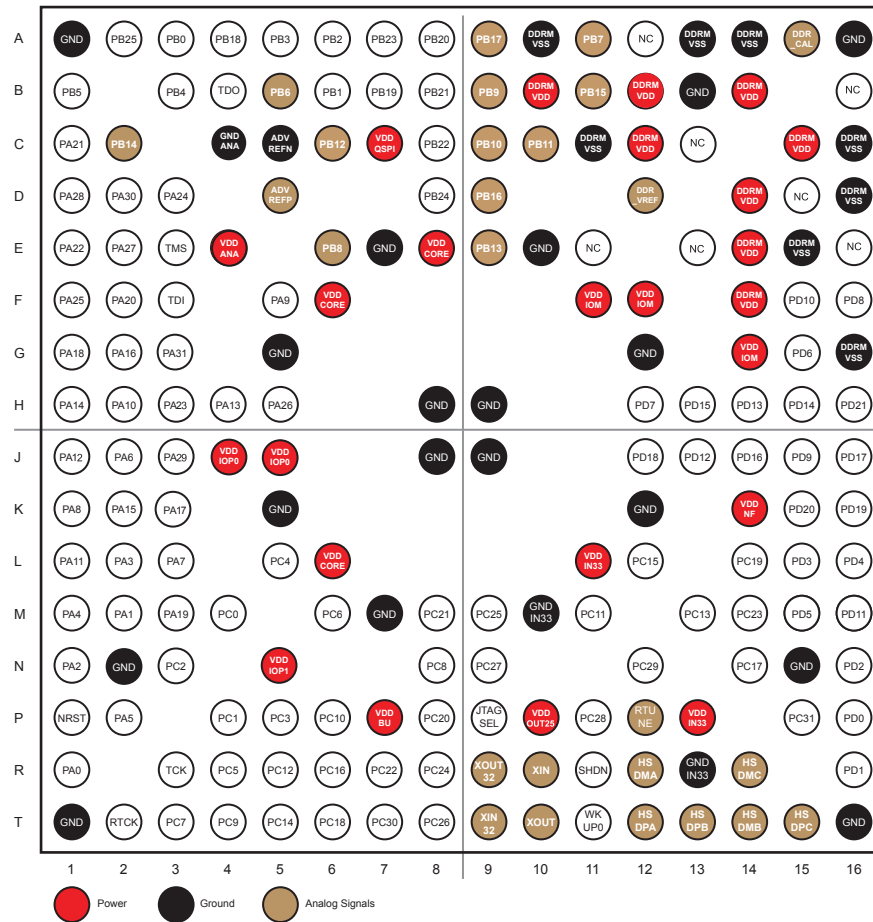
Figure 6-2. BGA196 Ballout
