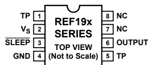
Figure 1. 8-Lead SOIC_N and TSSOP Pin Configuration (S Suffix and RU Suffix)
