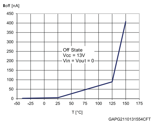
Figure 15: OFF-state output current
