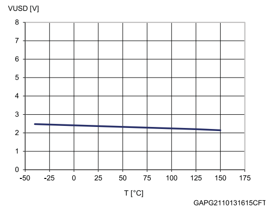
Figure 24: Undervoltage shutdown
