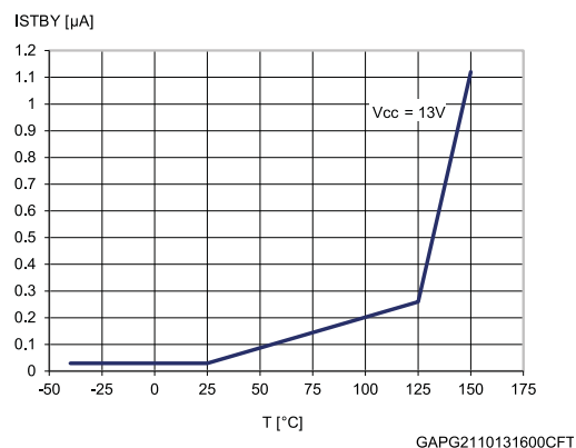
Figure 16: Standby current
