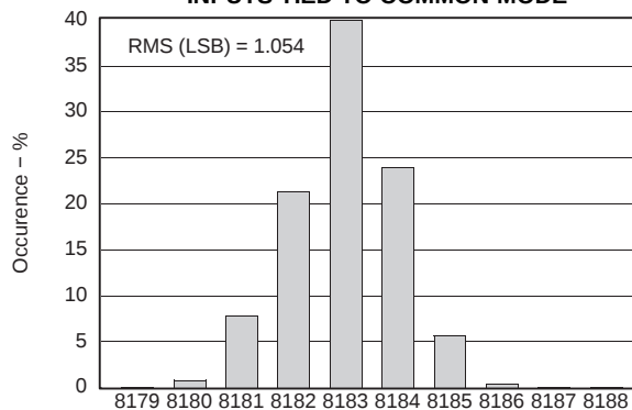
OUTPUT NOISE HISTOGRAM WITH INPUTS TIED TO COMMON-MODE
