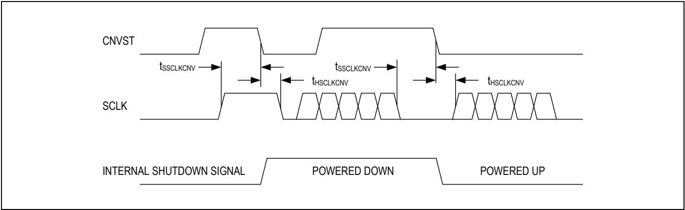
Figure 4. Entering and Exiting Shutdown Mode
