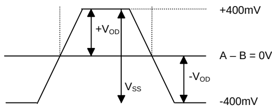
Figure 5: Single-ended and Differential Waveforms
