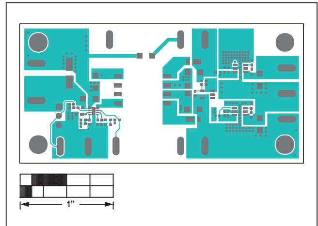
Figure 2. MAX17681V EV Kit PCB Layout—Component Side
