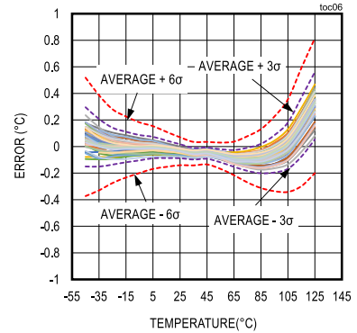
ACCURACY vs. TEMPERATURE ( V_{DD} = 3.6\text{V} 59UNITS)
