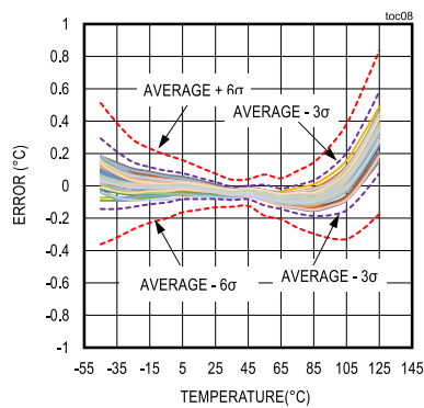
ACCURACY vs. TEMPERATURE ( V_{DD} = 3.3\text{V} 59UNITS)
