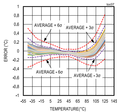
ACCURACY vs. TEMPERATURE ( V_{DD} = 3.0\text{V} 59UNITS)
