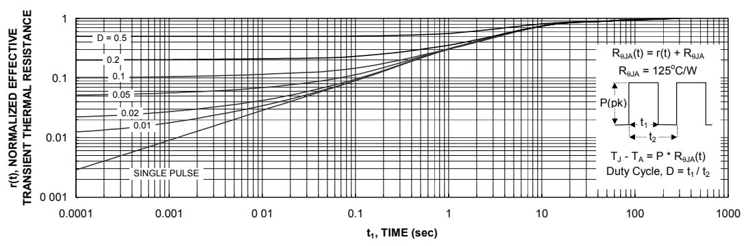
Figure 11. Transient Thermal Response Curve. Thermal characterization performed using the conditions described in Note 1c. Transient thermal response will change depending on the circuit board design.
