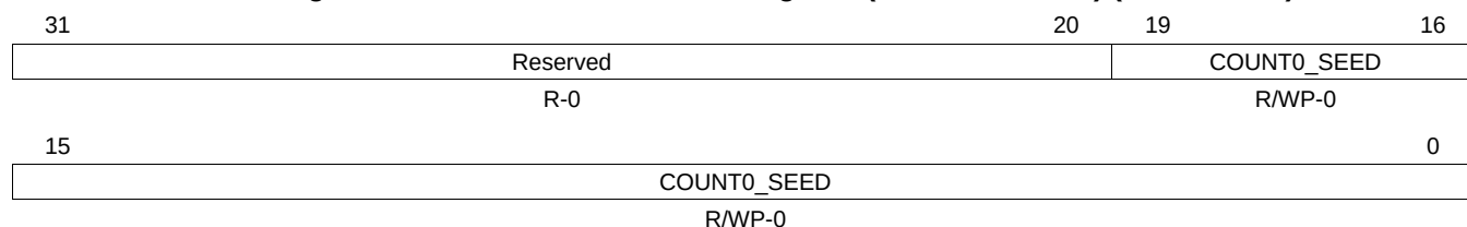
Figure 10-9. DCC Counter0 Seed Register (DCCCNT0SEED) (offset = 08h)
