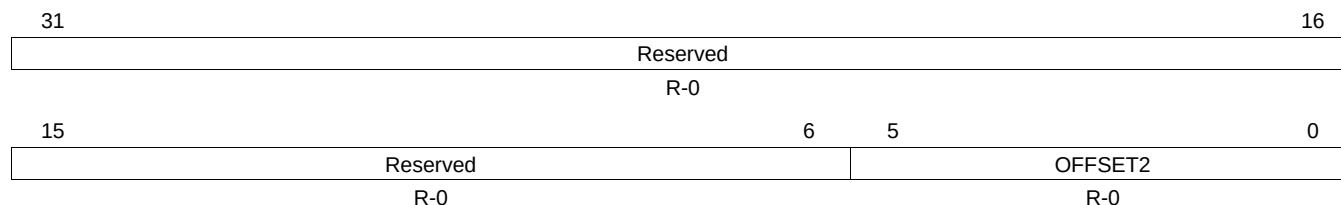
Figure 17-39. Offset Index Priority Level 2 Register (HETOFF2) [offset = 10h]
