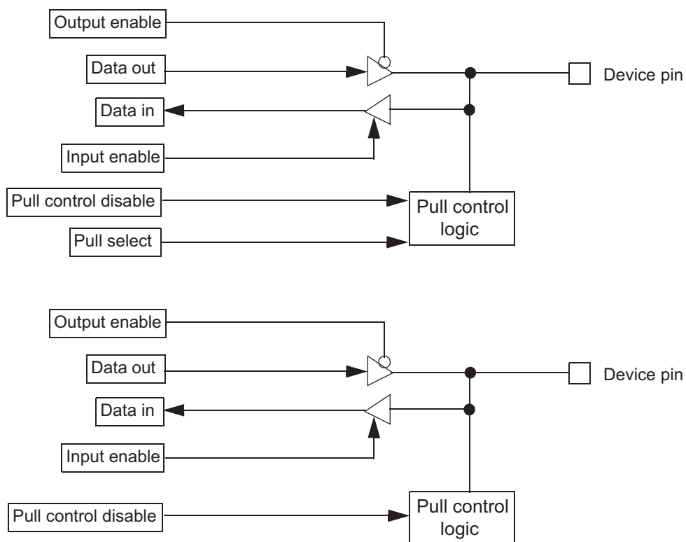
Figure 22-60. GPIO Functionality
