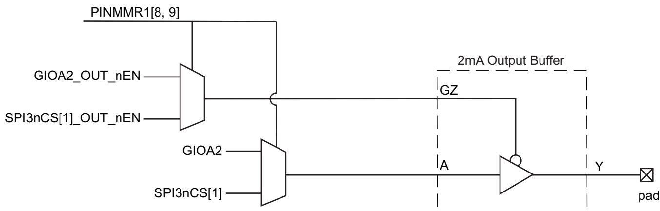
Figure 3-2. Output Multiplexing Example
