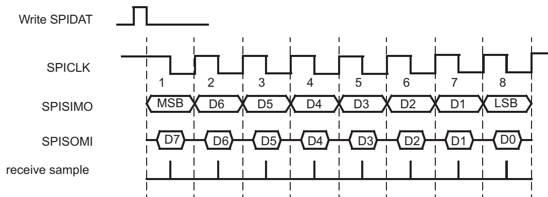
Figure 21-11. Clock Mode with Polarity = 1 and Phase = 1
