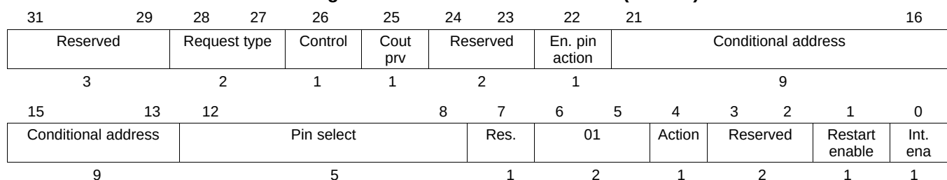
Figure 17-136. SCMP Control Field (C31:C0)
