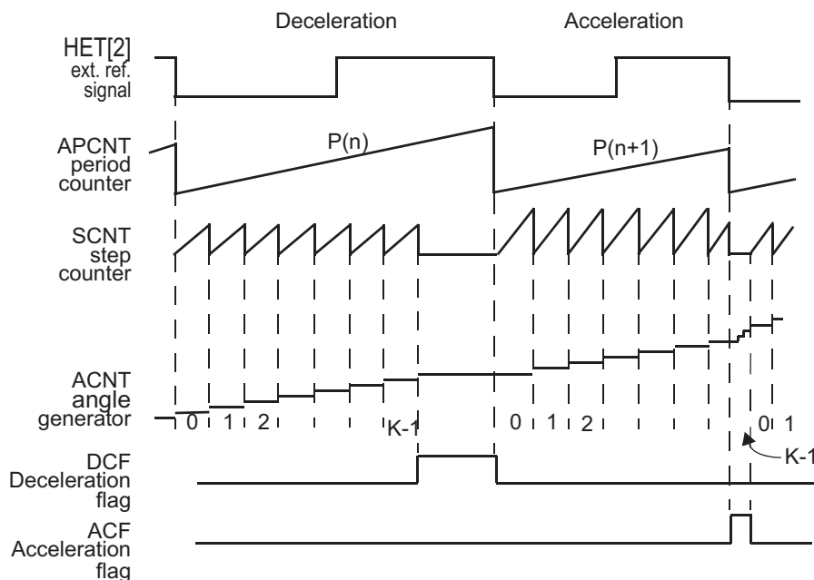
Figure 17-32. ACNT Period Variation Compensations
