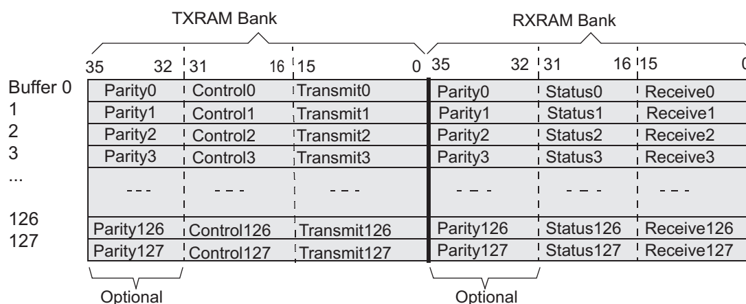
Figure 21-63. Multi-Buffer RAM Configuration
