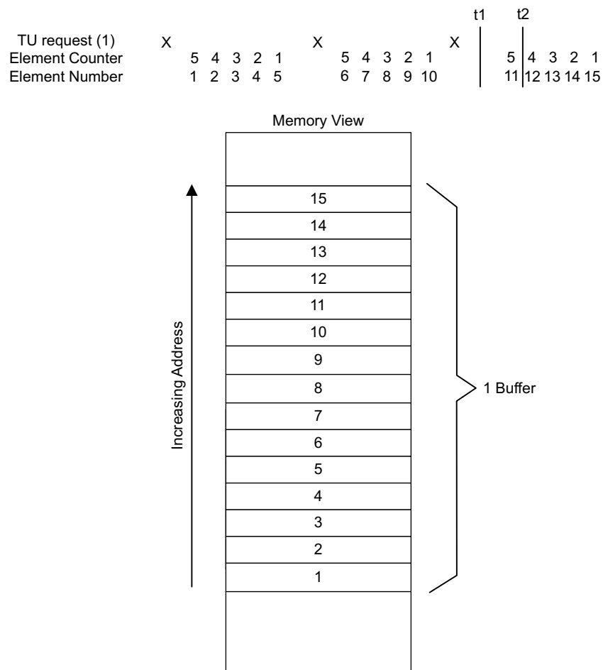
Figure 18-4. Single Buffer Timing and Memory Representation
