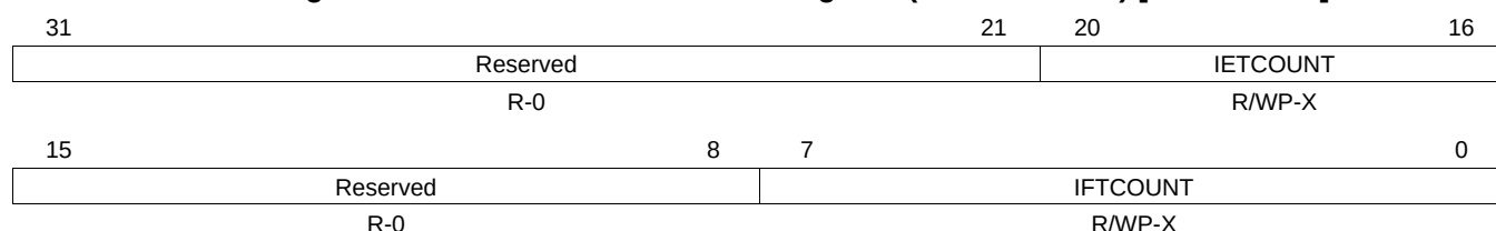
Figure 18-45. Initial Transfer Count Register (HTU ITCOUNT) [offset = 0Ch]
