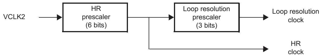
Figure 17-7. Prescaler Configuration
