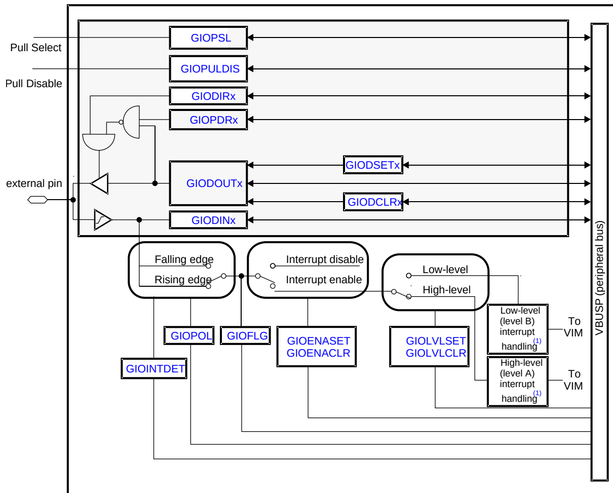
Figure 19-4. GIO Block Diagram
