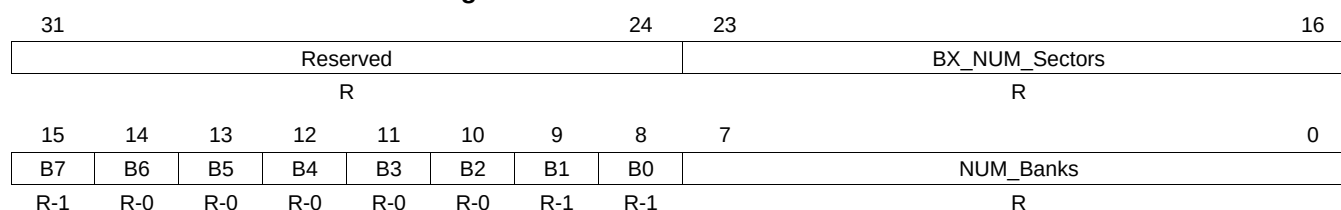
Figure 4-3. TI OTP Bank 0 Sector Information
