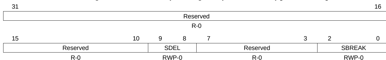
Figure 22-51. LIN Compare Register (LINCOMPARE) [offset = 60h]
