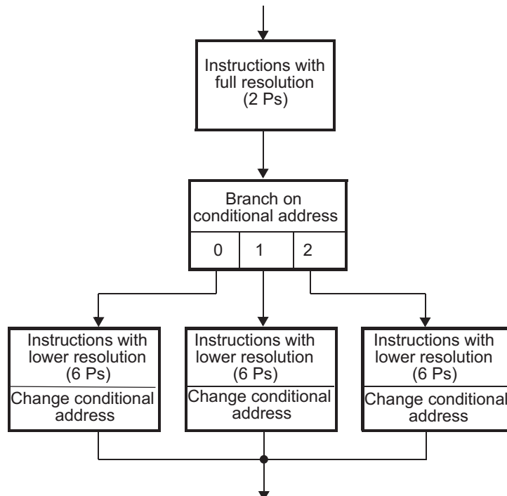
Figure 17-5. Multi-Resolution Operation Flow Example
