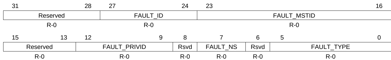
Figure 3-12. FAULT_STATUS_REG: Fault Status Register (Offset = F8h)
