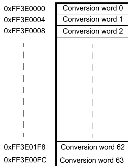
Figure 16-5. ADC Memory-Mapping
