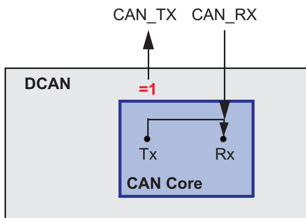
Figure 20-15. CAN Core in Silent Mode
