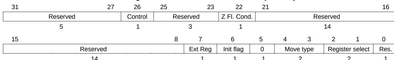
Figure 17-112. MOV32 Control Field (C31:C0)
