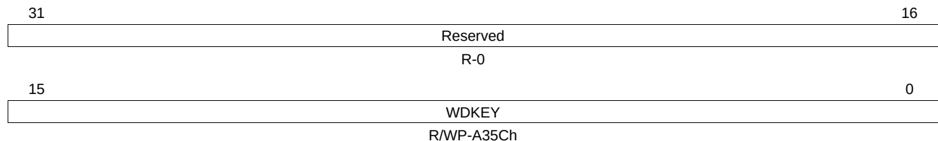
Figure 12-35. RTI Watchdog Key Register (RTIDWDKEY) [offset = 9Ch]
