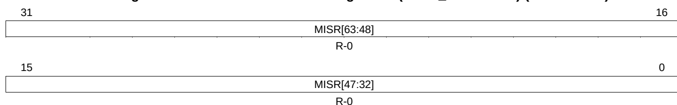
Figure 7-11. CPU1 Current MISR Register 2 (CPU1_CURMISR2) (offset = 20h)
