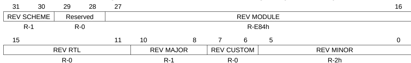
Figure 3-3. REVISION_REG: Revision Register (Offset = 00h)
