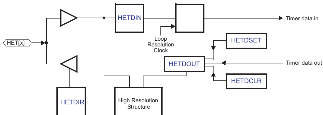
Figure 17-8. I/O Control
