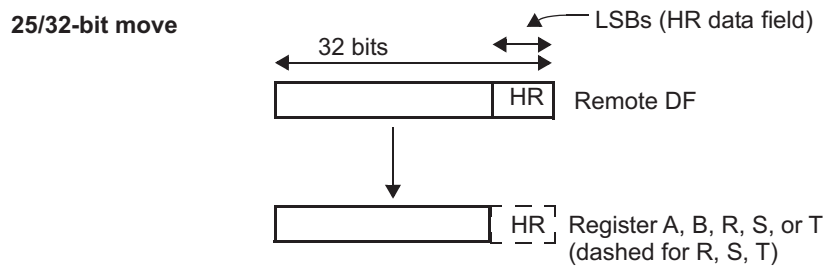
Figure 17-117. MOV32 Move Operation for REMTOREG (Case 11)
