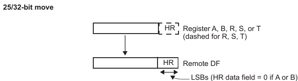
Figure 17-116. MOV32 Move Operation for REGTOREM (Case 10)
