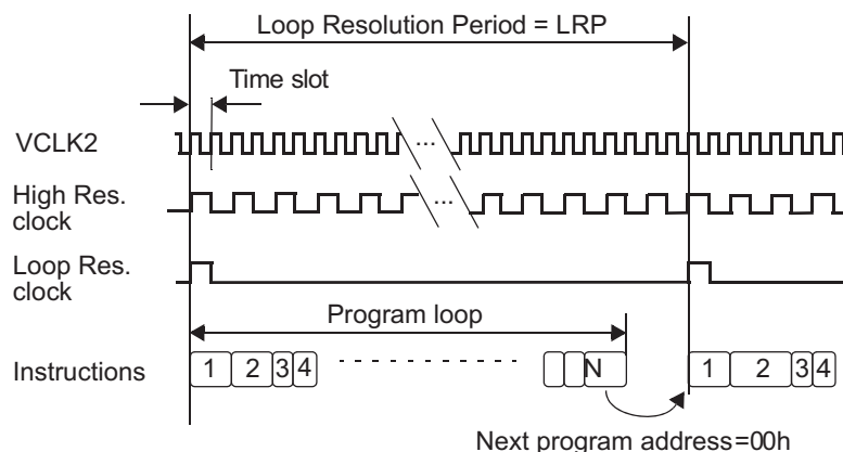
Figure 17-3. Program Flow Timings
