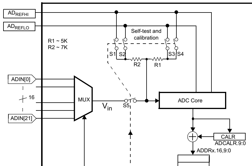
Figure 16-11. Self-Test and Calibration Logic
