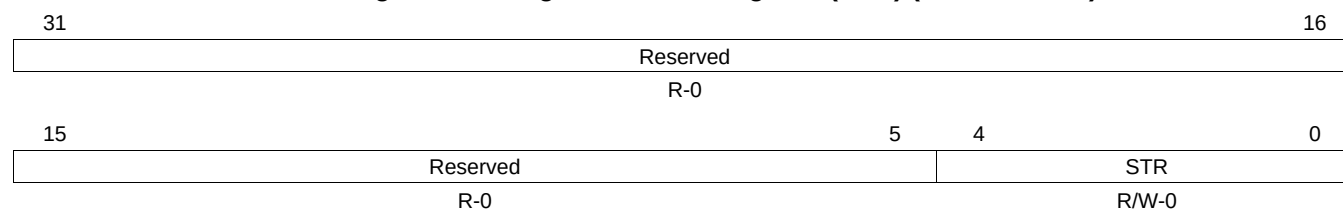
Figure 6-5. Program Control Register (PCR) (offset = 16Ch)
