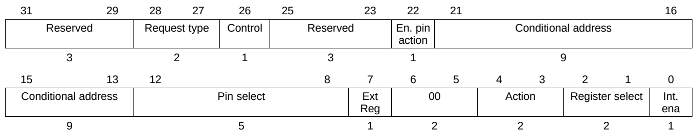
Figure 17-103. ECMP Control Field (C31:C0)
