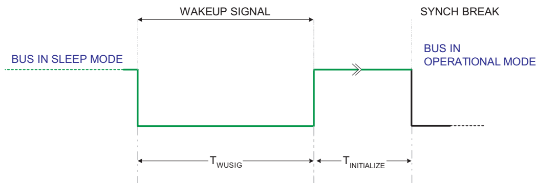
Figure 22-26. Wakeup Signal Generation
