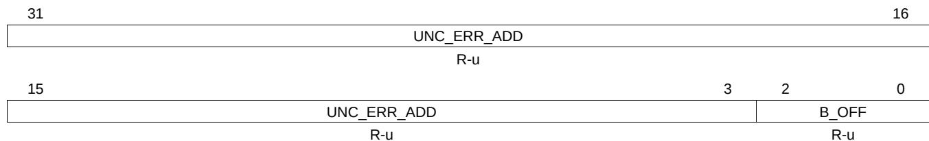
Figure 4-48. EEPROM Emulation Uncorrectable Error Address Register (EE_UNC_ERR_ADD) [offset = 320h]
