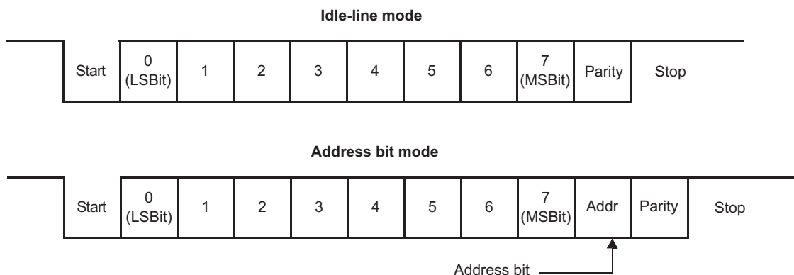
Figure 22-3. Typical SCI Data Frame Formats
