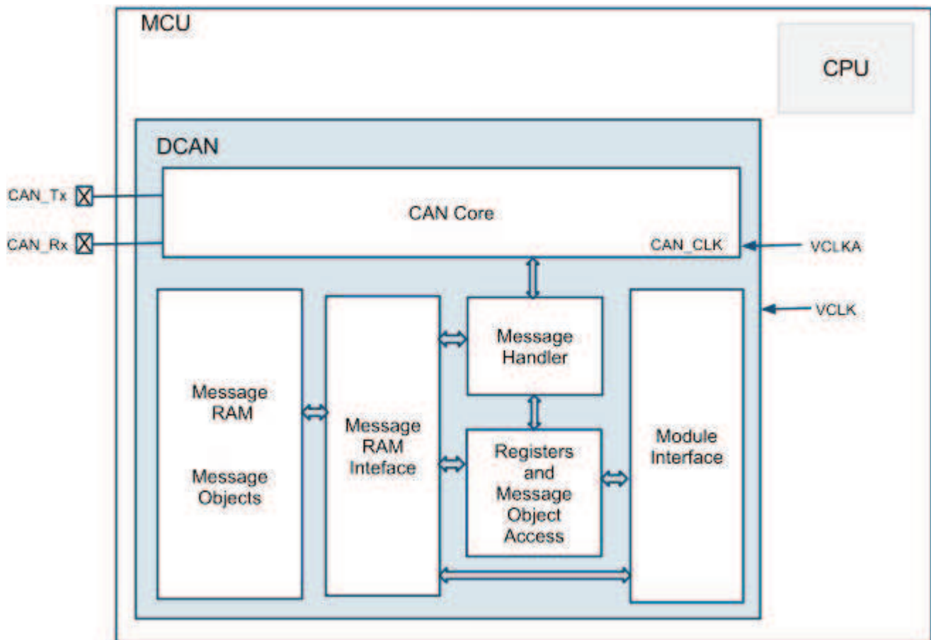
Figure 20-1. Block Diagram
