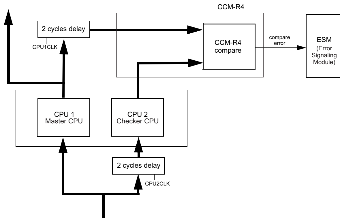
Figure 8-1. Block Diagram
