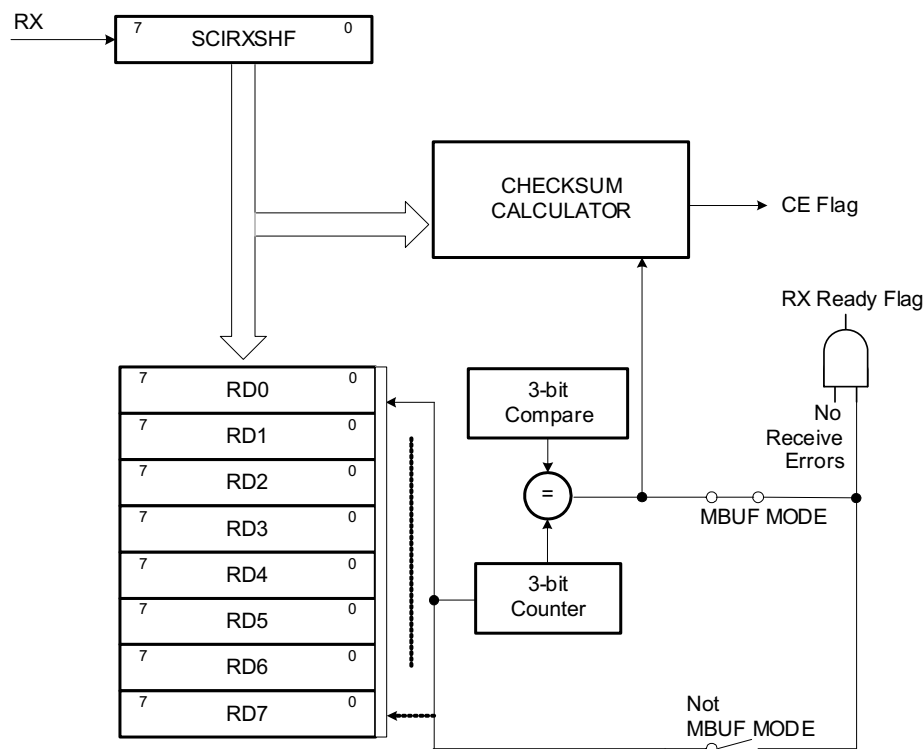
Figure 22-8. Receive Buffers
