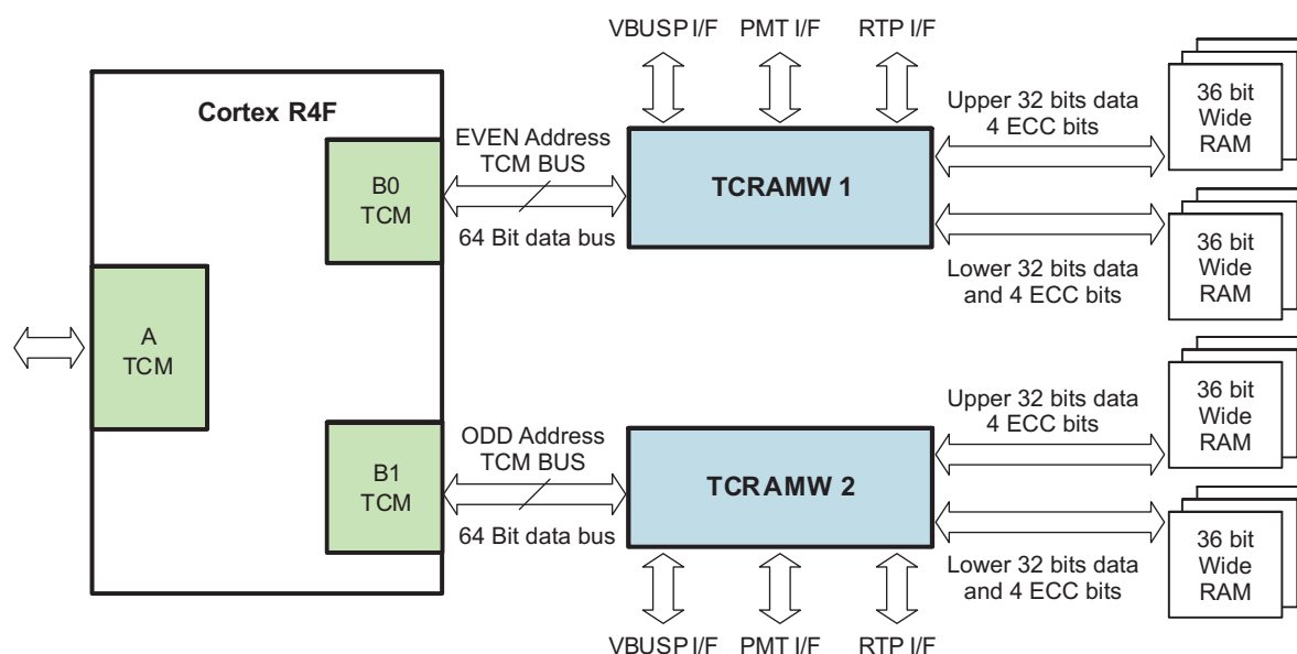
Figure 5-1. TCRAM Module Connections
