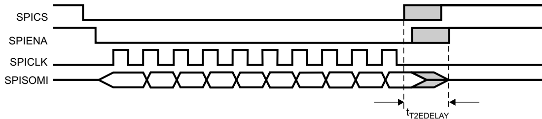
Figure 21-38. Transmit-Data-Finished-to-ENA-Inactive-Timeout
