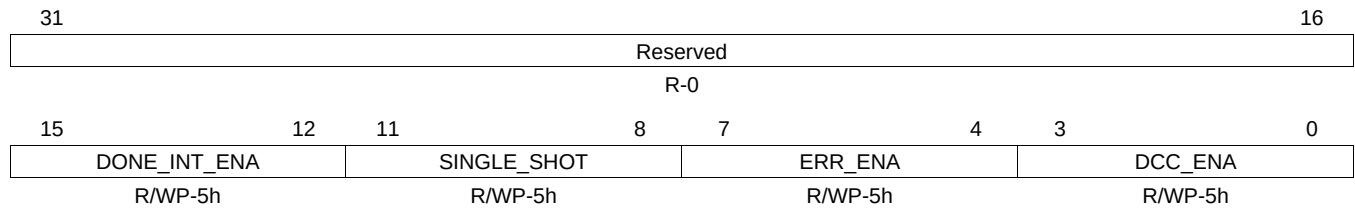
Figure 10-7. DCC Global Control Register (DCCGCTRL) (offset = 00h)
