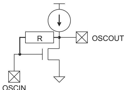
Figure 9-3. Oscillator Implementation
