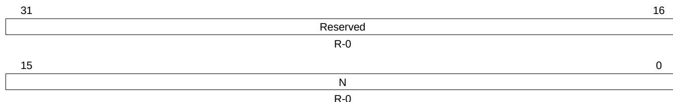
Figure 7-7. STC Current Interval Count Register (STCCICR) (offset = 10h)
