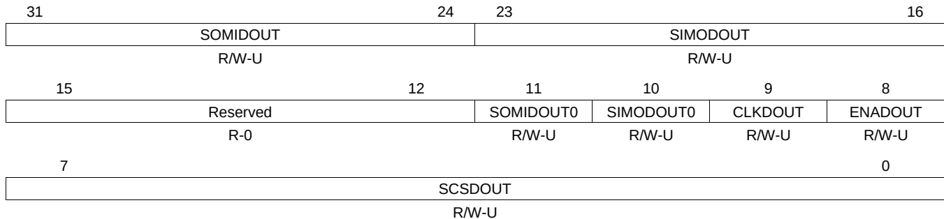
Figure 21-25. SPI Pin Control Register 3 (SPIPC3) [offset = 20h]
