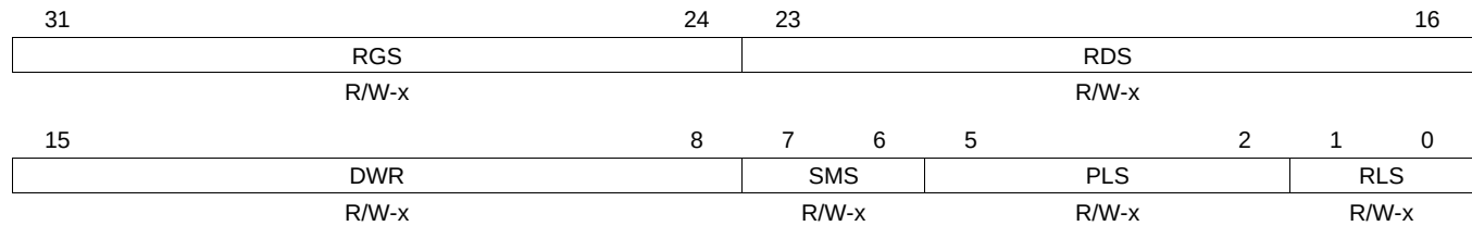
Figure 6-3. RAM Configuration Register (RAMT) (offset = 160h)
