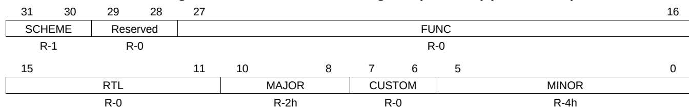
Figure 10-8. DCC Revision ID Register (DCCREV) (offset = 04h)
