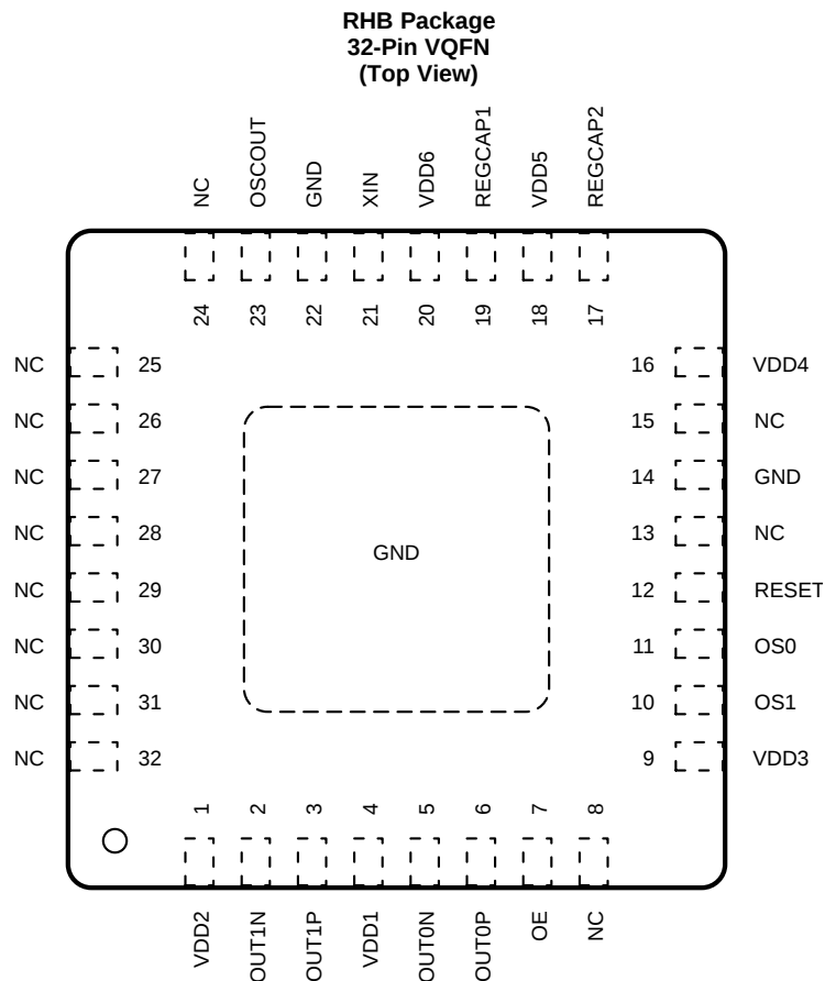
Pin Functions
