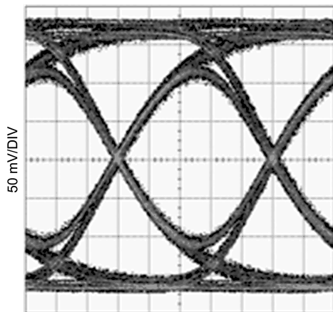
Figure 23. Equalized Signal (Zoom) (30in FR4, 5Gbps, PRBS7)
