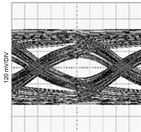
Figure 24. Unequalized Signal (34in Tyco XAUI Backplane, 3.125Gbps, PRBS7)
