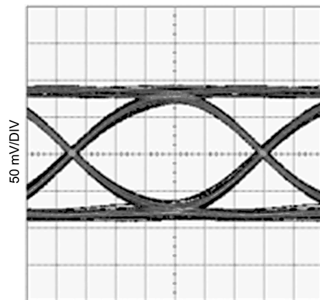
Figure 26. Equalized Signal (Zoom) (34in Tyco XAUI Backplane, 3.125Gbps, PRBS7)
