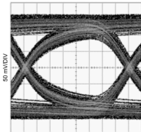
Figure 35. Equalized Signal (Zoom) (10m 24AWG PCIe Cable, 2.5Gbps, PRBS7)
