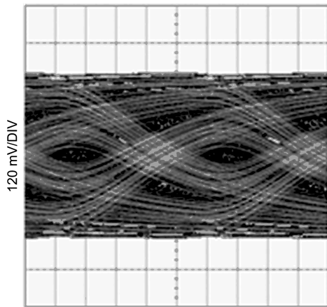
Figure 21. Unequalized Signal (30in FR4, 5Gbps, PRBS7)
