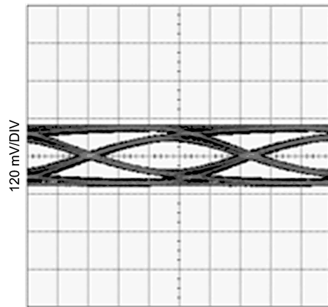
Figure 16. Equalized Signal (40in FR4, 3.8Gbps, PRBS7)
