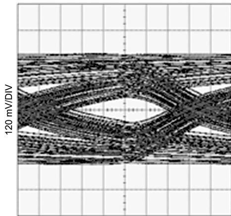
Figure 33. Unequalized Signal (10m 24AWG PCIe Cable, 2.5Gbps, PRBS7)
