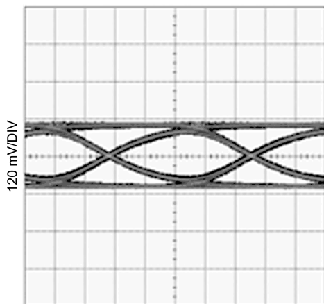
Figure 19. Equalized Signal (30in FR4, 4.25Gbps, PRBS7)
