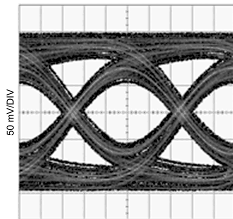
Figure 38. Equalized Signal (Zoom) (10m 24AWG PCIe Cable, 5Gbps, PRBS7)
