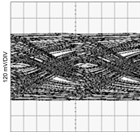
Figure 15. Unequalized Signal (40in FR4, 3.8Gbps, PRBS7)
