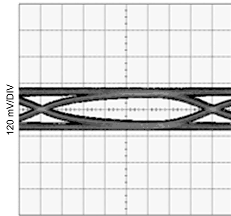
Figure 34. Equalized Signal (10m 24AWG PCIe Cable, 2.5Gbps, PRBS7)
