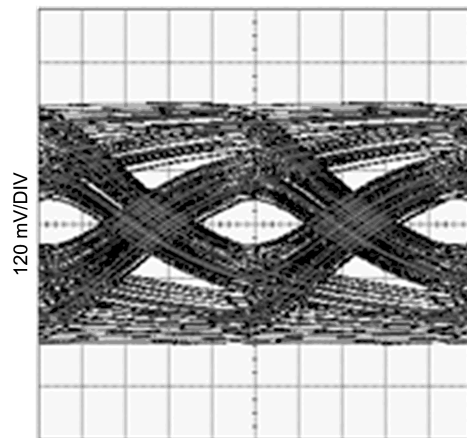
Figure 18. Unequalized Signal (30in FR4, 4.25Gbps, PRBS7)
