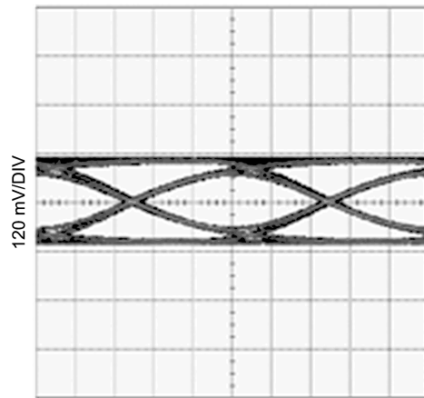
Figure 22. Equalized Signal (30in FR4, 5Gbps, PRBS7)
