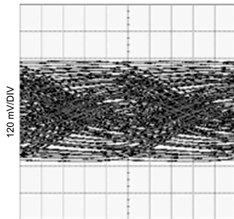
Figure 36. Unequalized Signal (10m 24AWG PCIe Cable, 5Gbps, PRBS7)
