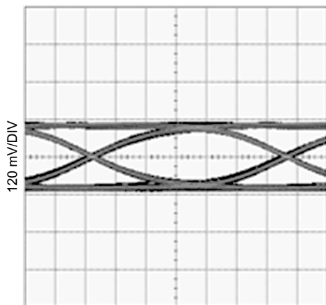
Figure 25. Equalized Signal (34in Tyco XAUI Backplane, 3.125Gbps, PRBS7)
