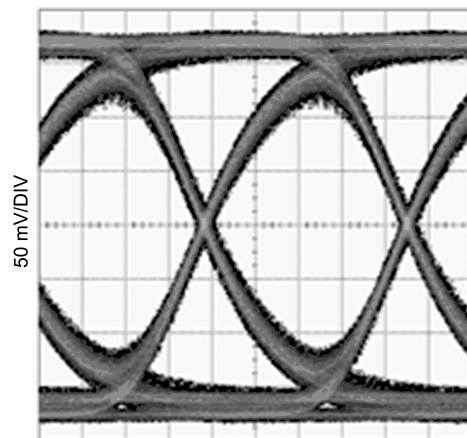
Figure 20. Equalized Signal (Zoom) (30in FR4, 4.25Gbps, PRBS7)
