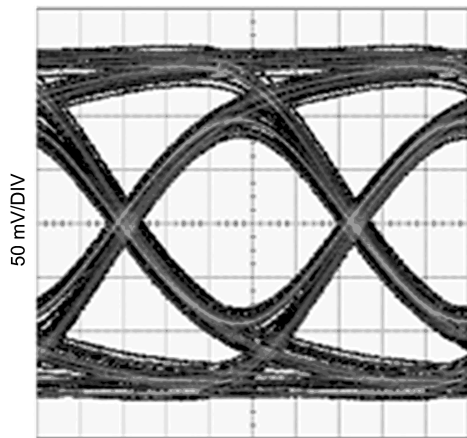
Figure 17. Equalized Signal (Zoom) (40in FR4, 3.8Gbps, PRBS7)
