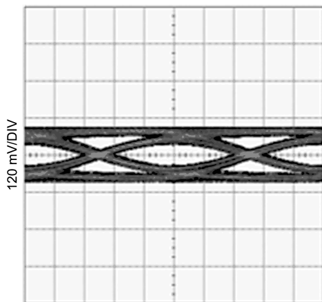
Figure 37. Equalized Signal (10m 24AWG PCIe Cable, 5Gbps, PRBS7)
