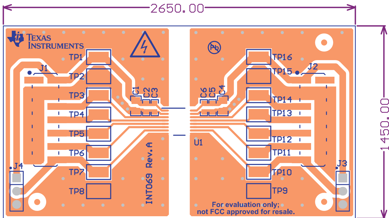
Figure 8. ISO7741DBQ PCB Layout
