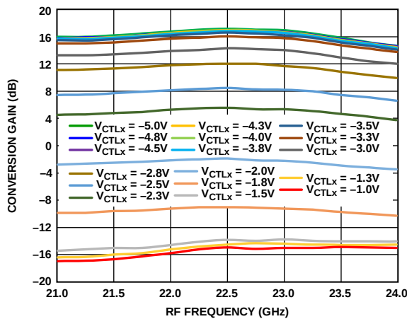
Figure 16. Conversion Gain vs. RF Frequency at Various Control Voltages, LO = 4 dBm
