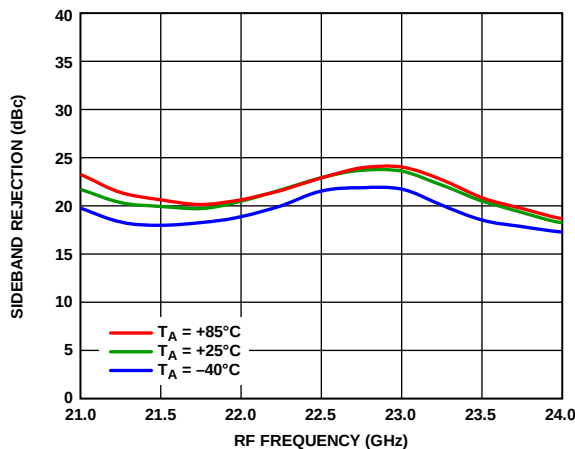
Figure 17. Sideband Rejection vs. RF Frequency at Various Temperatures, LO = 4 dBm
