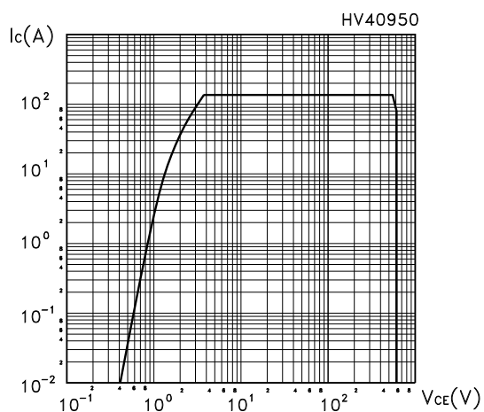
Figure 13. Turn-off SOA
