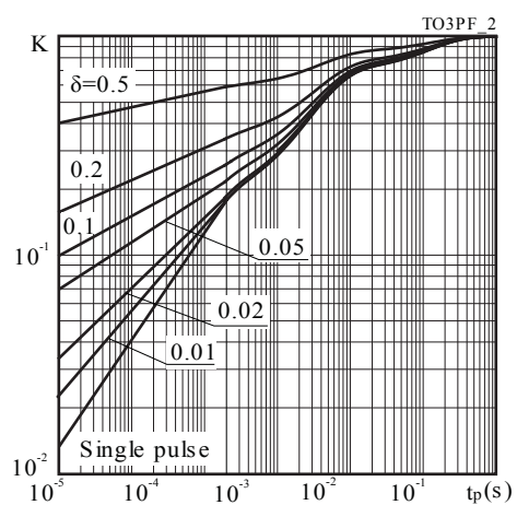
Figure 14. Thermal Impedance
