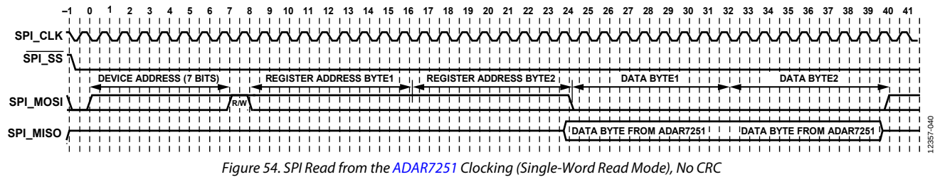
Figure 54. SPI Read from the ADAR7251 Clcking (Single-Word Read Mode), No CRC
