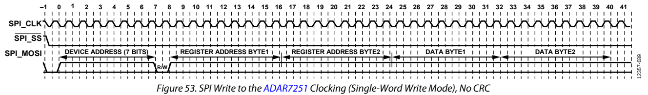
Figure 53. SPI Write to the ADAR7251 Clcking (Single-Word Write Mode), No CRC
