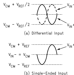
Figure 32. Expected Input Signal Range
