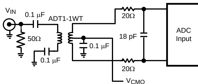
Figure 34. Low Input Frequency Transformer Drive Circuit
