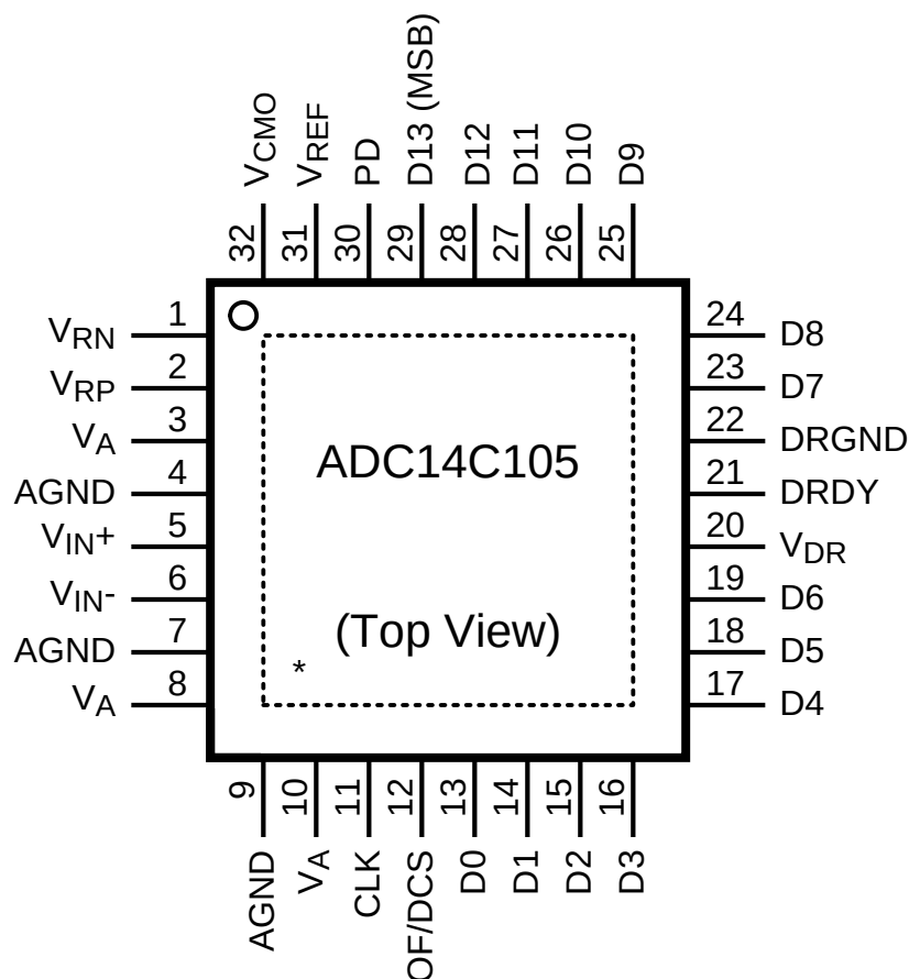
Figure 1. WQFN Package See Package Number RTV0032A
