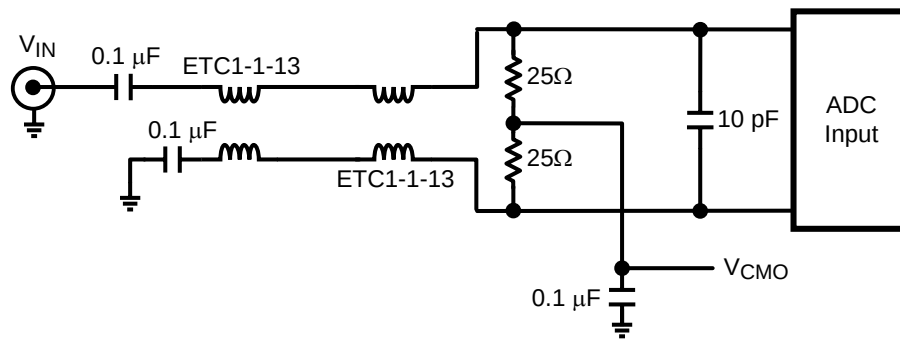
Figure 35. High Input Frequency Transformer Drive Circuit
