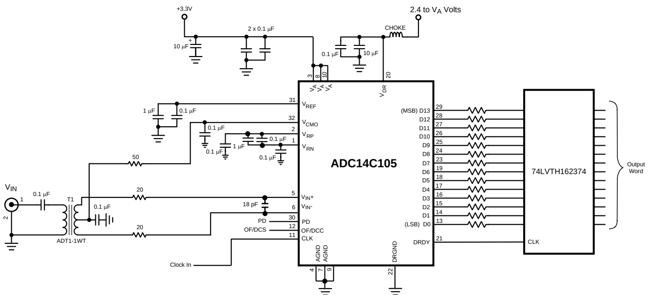
Figure 36. Application Circuit
