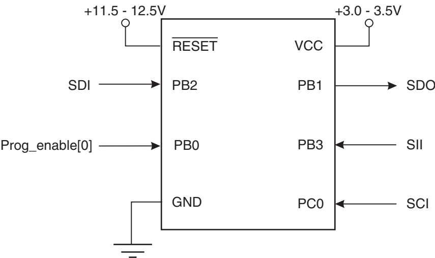
Figure 27-3. High-voltage Serial Programming
