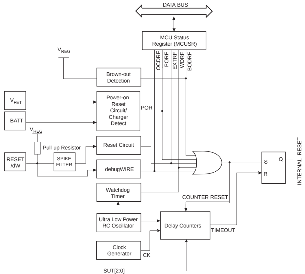
Figure 11-1. Reset Logic
