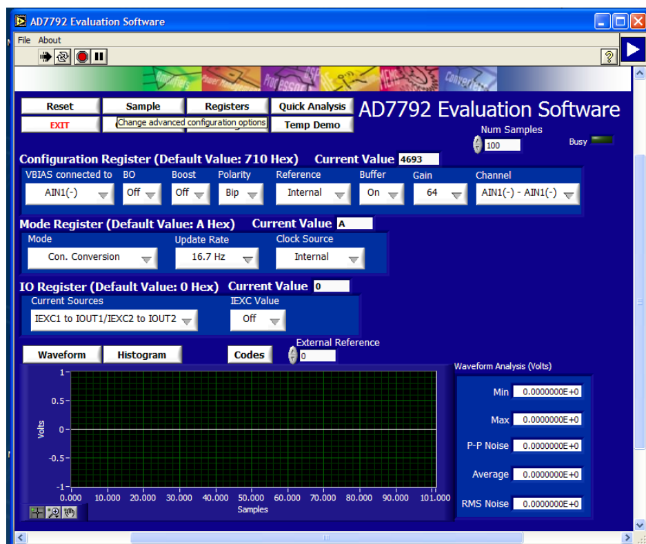
Figure 4. AD7792 Evaluation Software Registers Window
