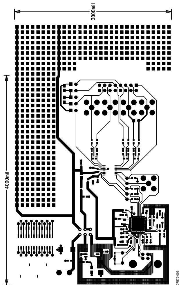
Figure 8. AD7792 Evaluation Board—Solder Side View
