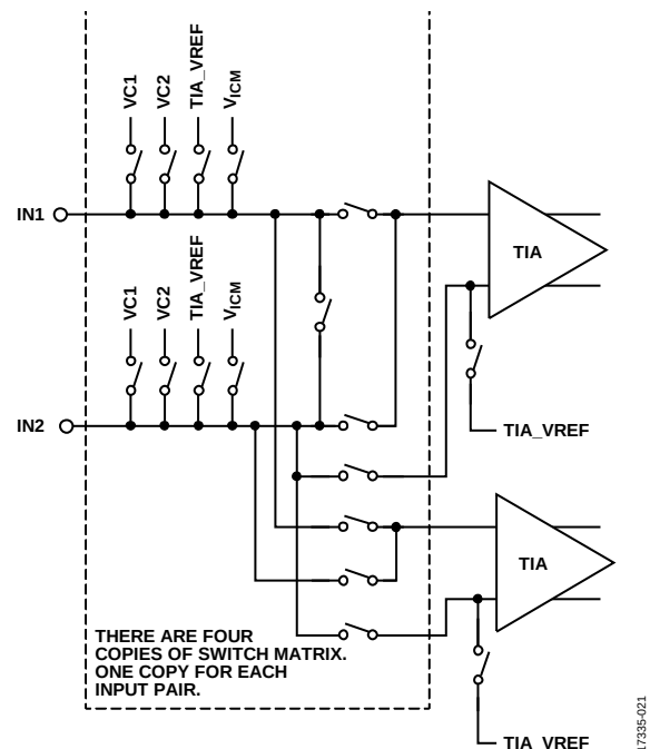
Figure 17. Analog Input Multiplexer
