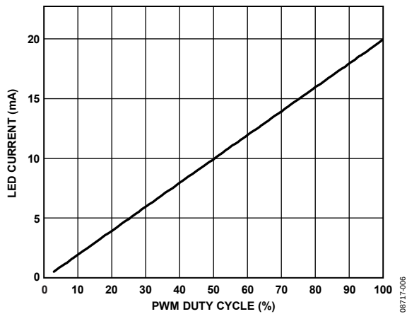
Figure 6. LED Current vs. PWM Input Duty Cycle
