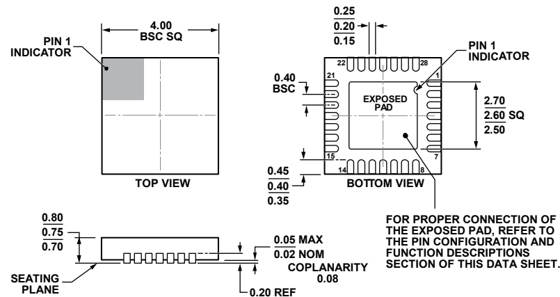
COMPLIANT TO JEDEC STANDARDS MO-220-WGGE. Figure 28. 28-Lead Lead Frame Chip Scale Package [LFCSP_WQ] 4 mm × 4 mm × 0.75 mm Body, Very Very Thin Dual (CP-28-5) Dimensions shown in millimeters
