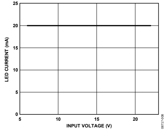
Figure 8. LED Current vs. Input Voltage ( I_{LED} = 20 \text{ mA} )
