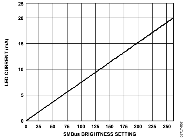
Figure 7. LED Current vs. SMBus Brightness Setting
