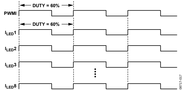
Figure 17. Direct PWM Dimming Timing
