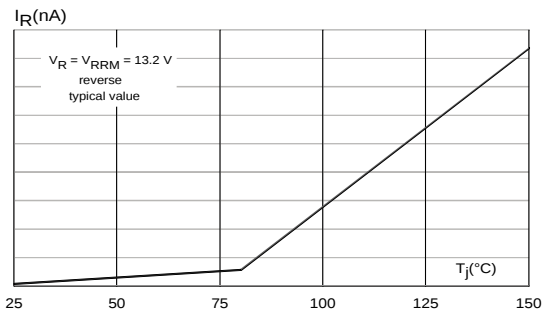
Figure 6: Leakage current versus junction temperature (typical value)
