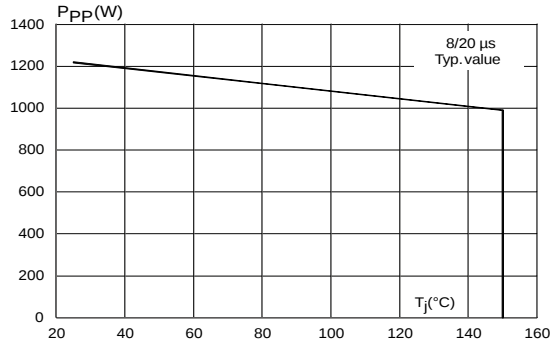
Figure 3: Peak power dissipation versus initial temperature (typ. value)
