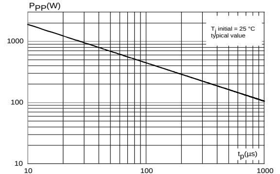
Figure 4: Peak pulse power versus exponential pulse duration ( T_J initial = 25°C) (typ. value)
