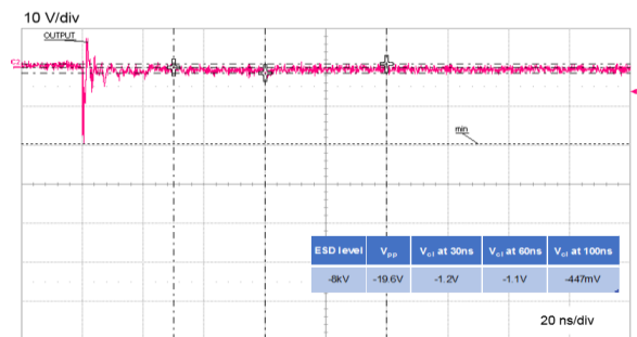
Figure 8: ESD response to IEC 61000-4-2 (-8kV contact discharge)
