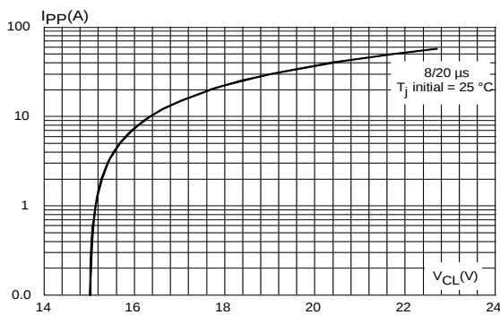
Figure 5: Clamping voltage versus peak pulse current (max. value)
