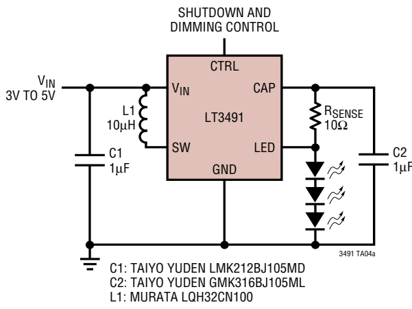
Li-Ion Driver for Three White LEDs
