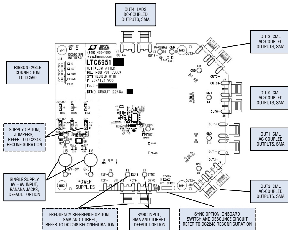
Figure 1. DC2248A Connections
