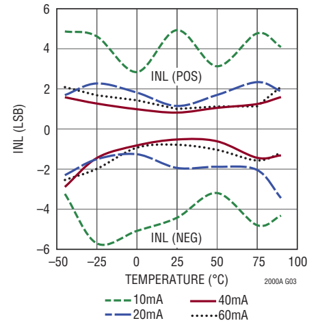
INL vs I_{OUTFS} and Temperature
