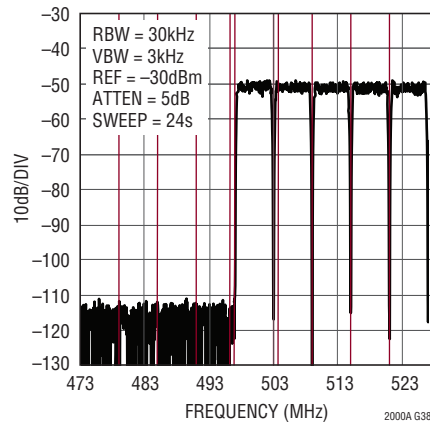
32 Carrier DOCSIS Mid Band Narrowband ACLR, f_{DAC} = 2.7Gsps
