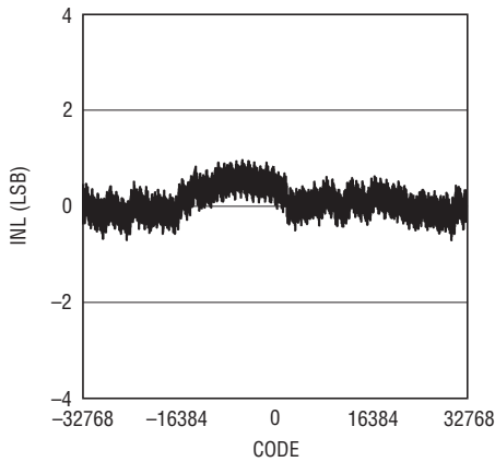
LTC2000A-16 Integral Nonlinearity (INL)
