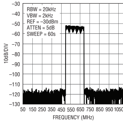
32-Carrier DOCSIS Mid Band Wideband ACLR, f_{DAC} = 2.7Gsps
