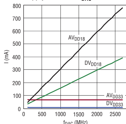
Supply Current vs f_{DAC}
