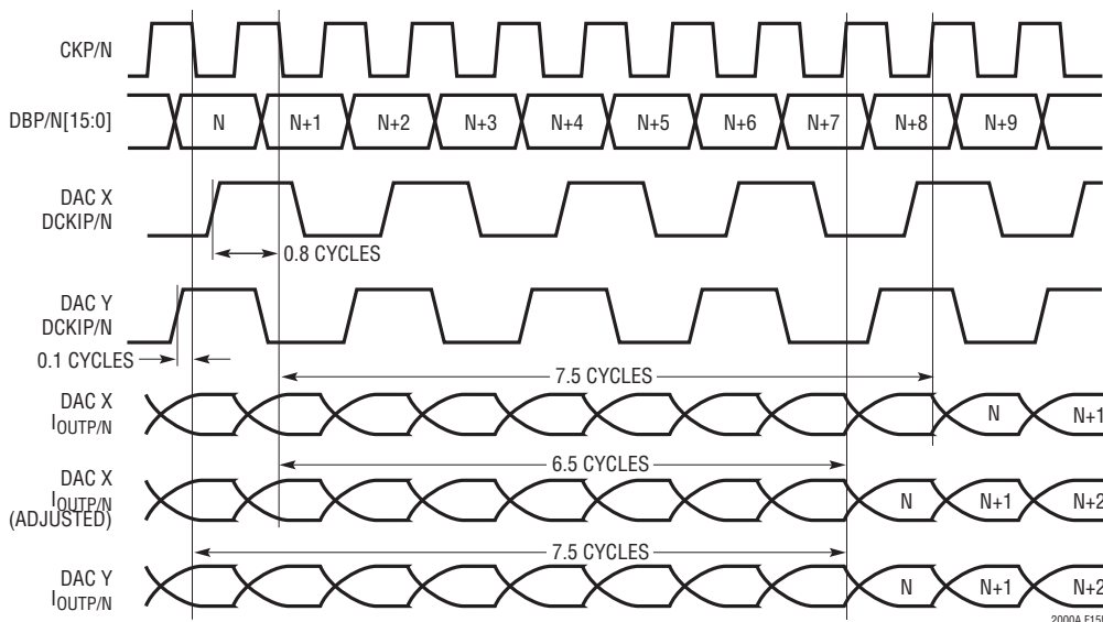
Figure 15b. Sample Waveforms — Synchronizing Multiple LTC2000As in Single Port Mode
