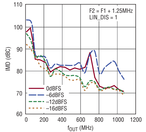
2-Tone IMD vs f_{OUT} and Digital Amplitude, f_{DAC} = 2.7\text{Gpsps}
