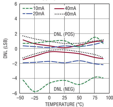
DNL vs I_{OUTFS} and Temperature
