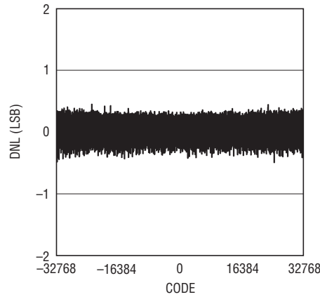
LTC2000A-16 Differential Nonlinearity (DNL)
