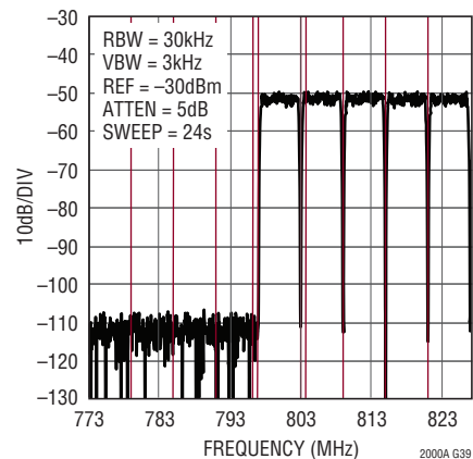
32 Carrier DOCSIS High Band Narrowband ACLR, f_{DAC} = 2.7Gsps
