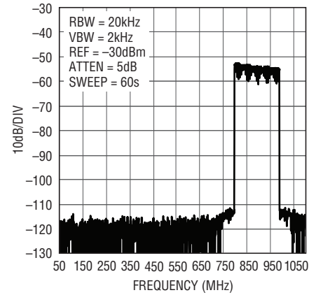
32 Carrier DOCSIS High Band Wideband ACLR, f_{DAC} = 2.7Gsps
