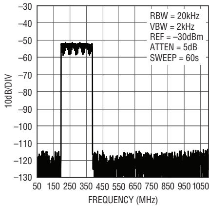
32-Carrier DOCSIS Low Band Wideband ACLR, f_{DAC} = 2.7Gsps
