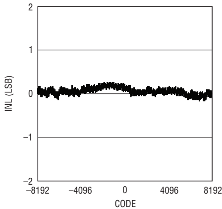
LTC2000A-14 Integral Nonlinearity (INL)
