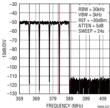
32-Carrier DOCSIS Low Band Narrowband ACLR, f_{DAC} = 2.7Gsps
