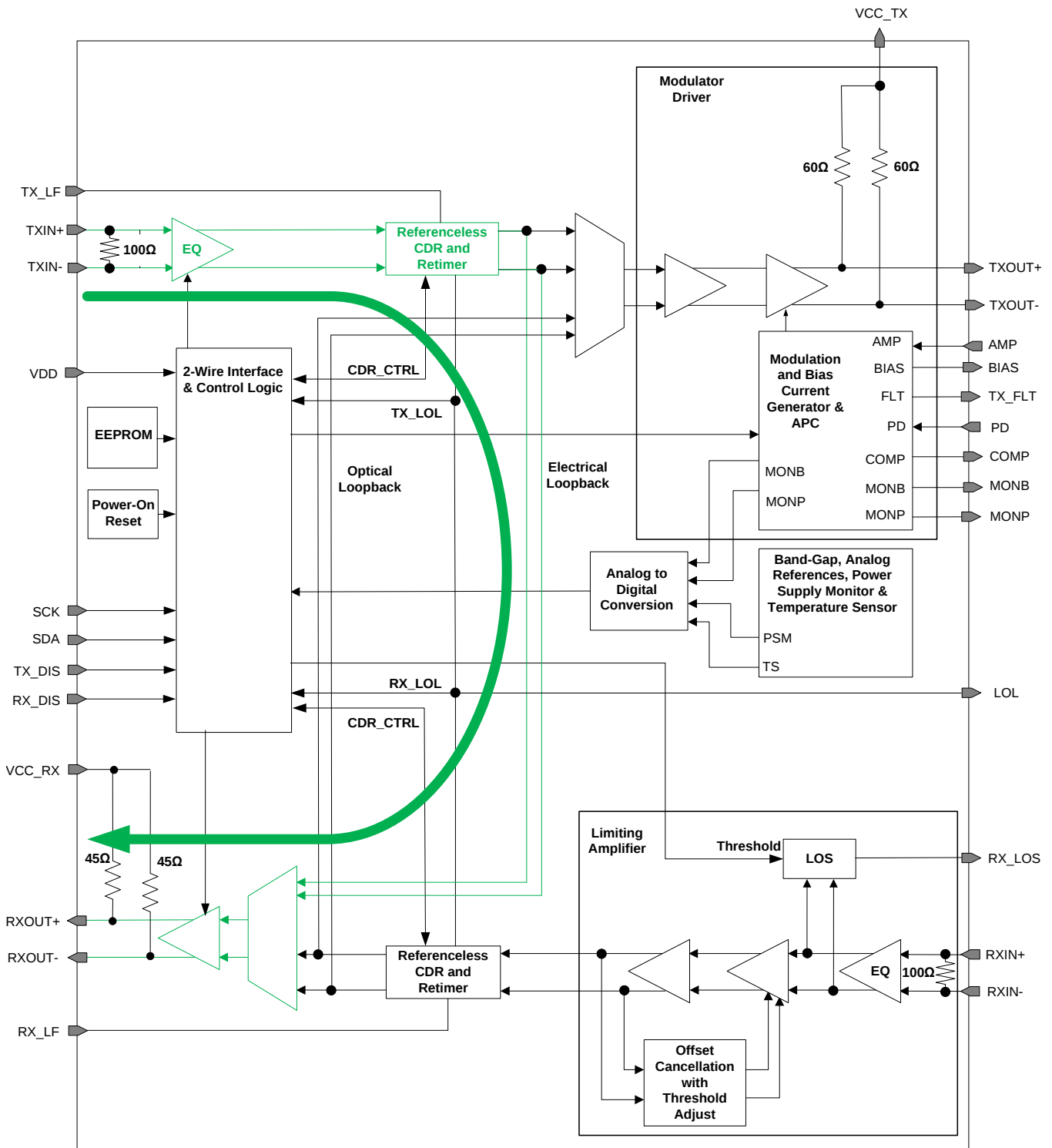
Figure 38. Electrical Loopback
