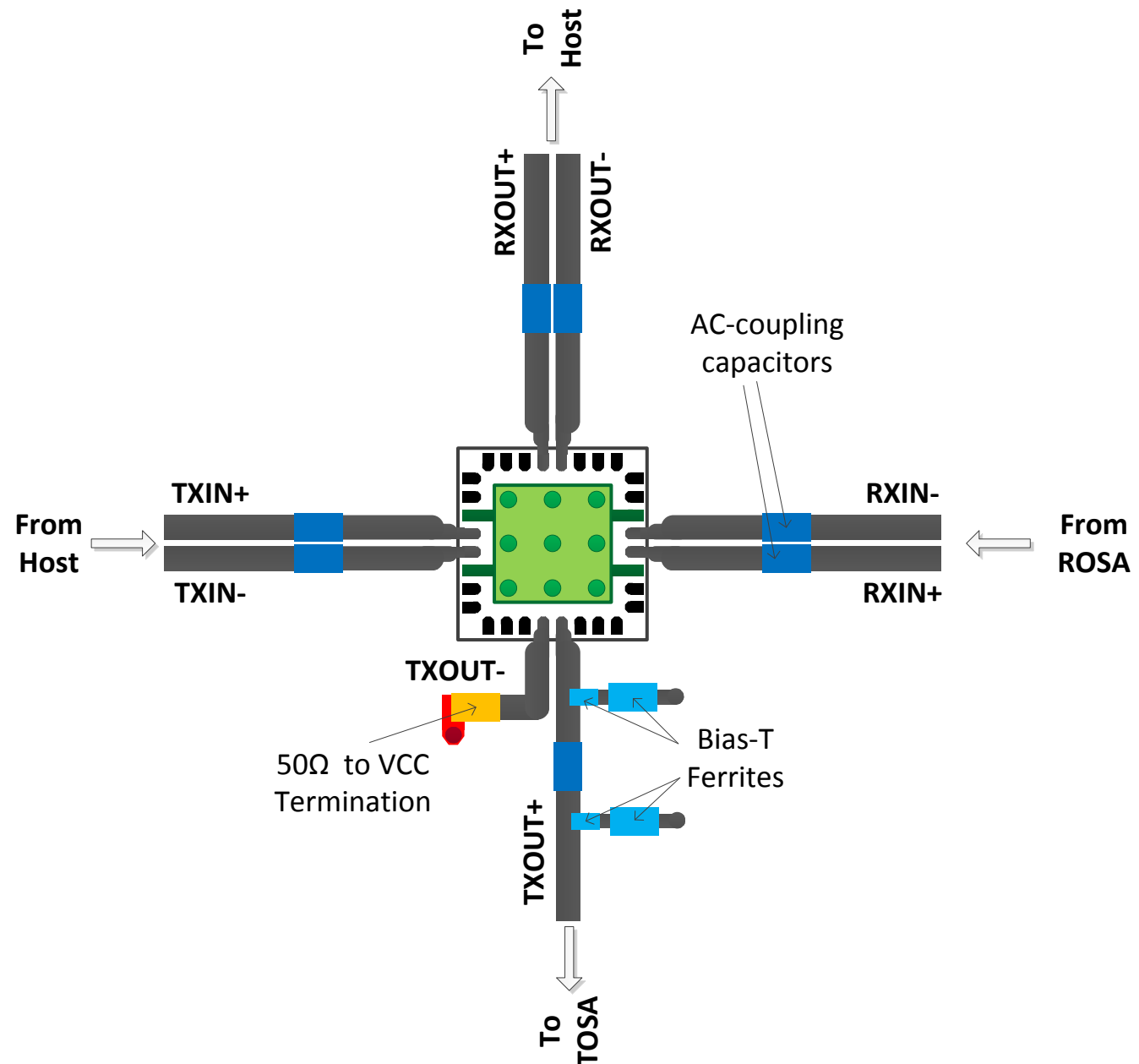
Figure 73. Board Layout
