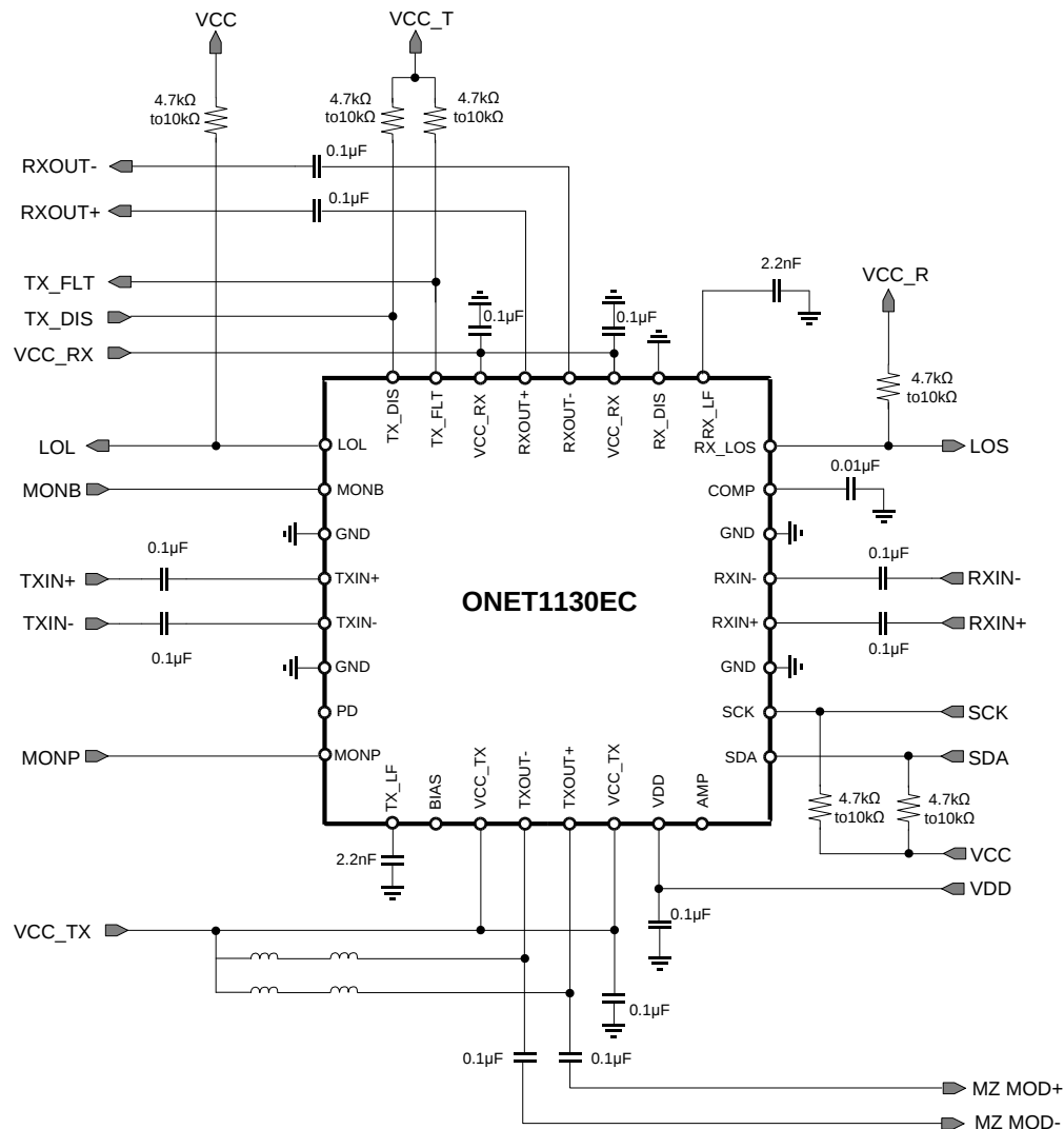
Figure 68. Typical Application Circuit in Differential Mode
