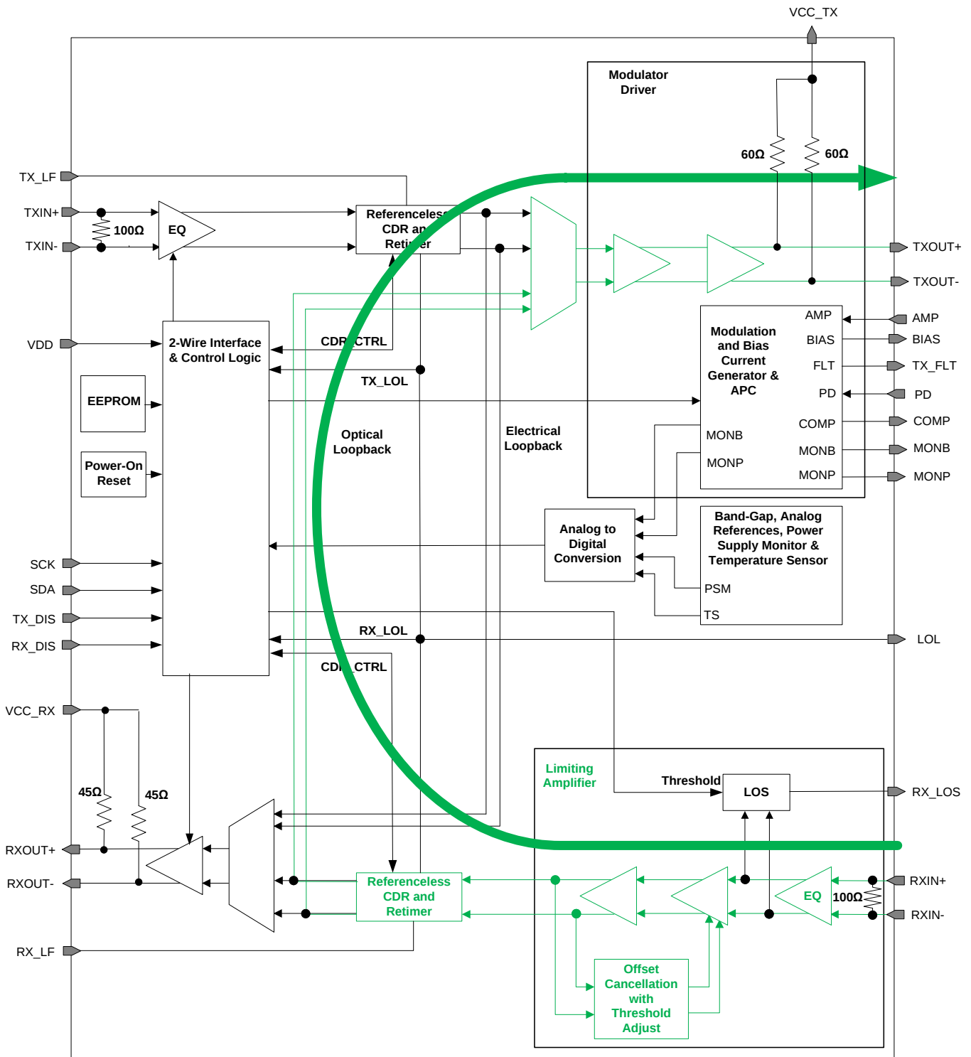
Figure 39. Optical Loopback
