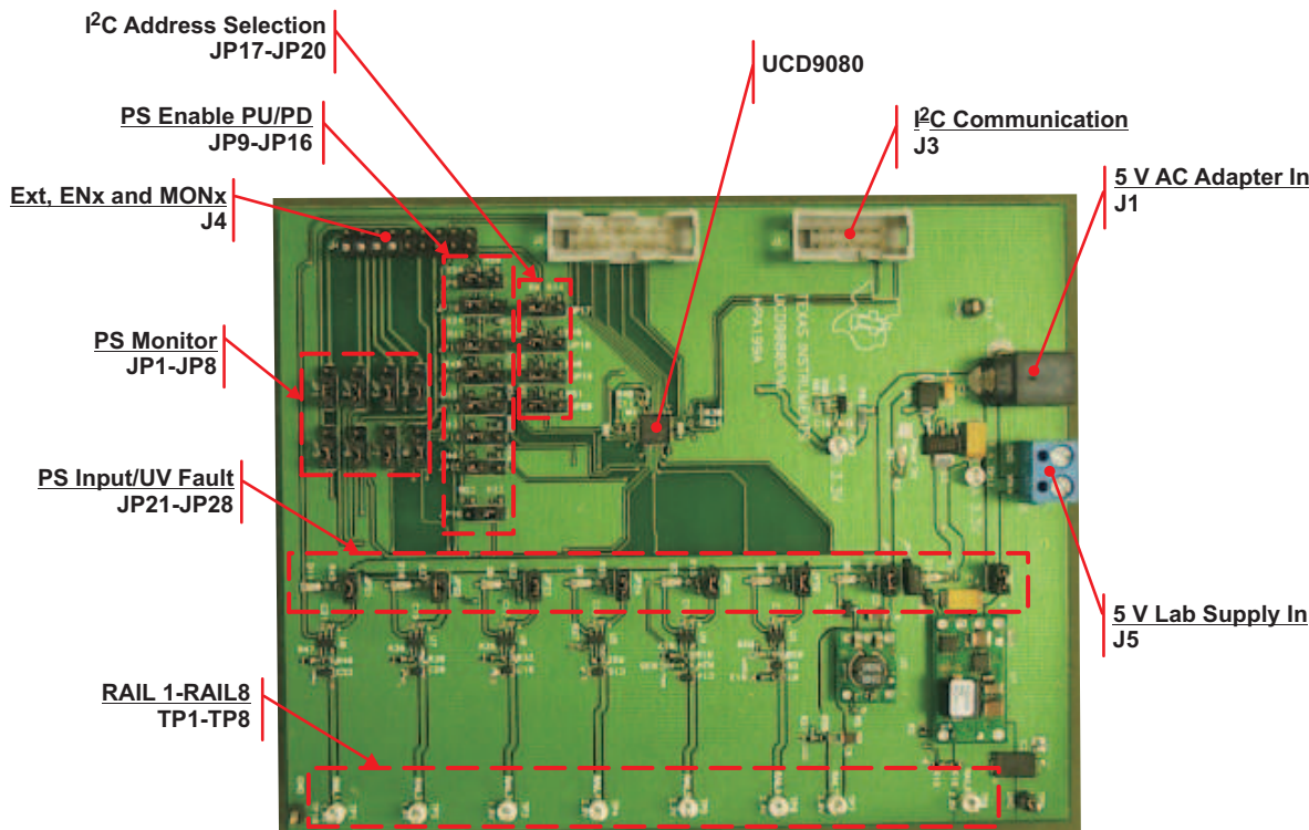
Figure 2. UCD9081EVM Functionality
