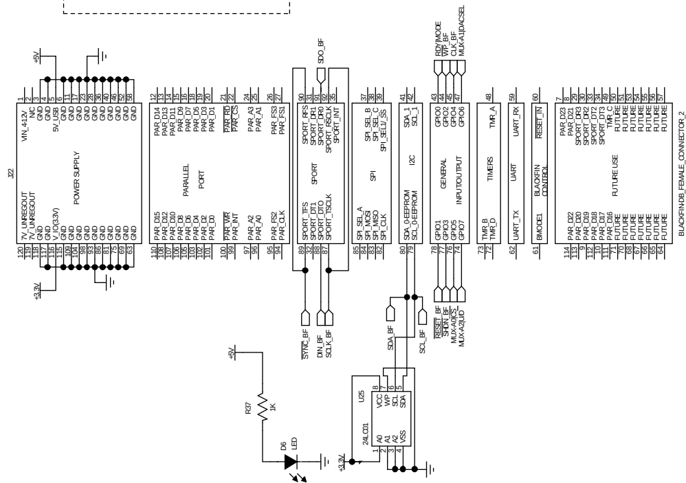
Figure 13. Schematic of SDP-B Connector
