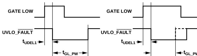
Figure 26. \overline{\text{UVLO\_FAULT}} Fault for V_{\text{DD2}} UVLO
