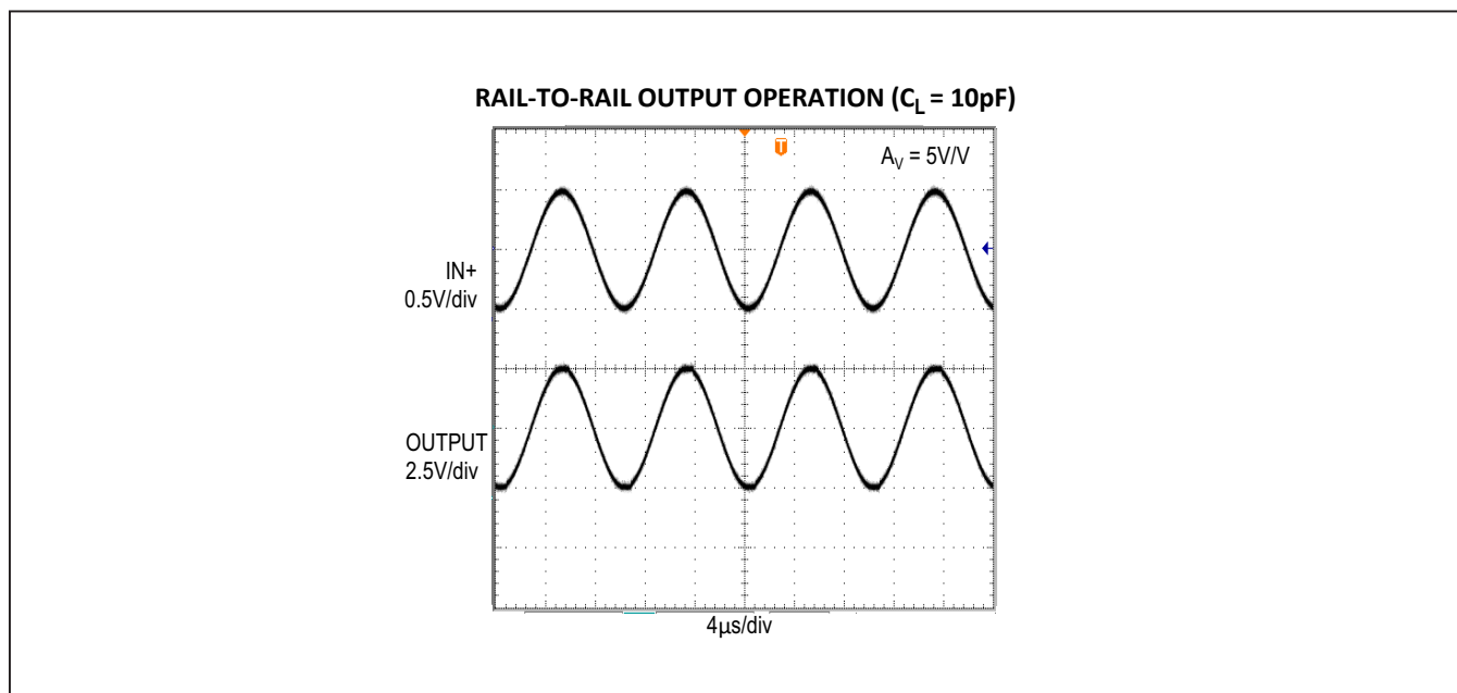
Figure 4. Rail-to-Rail Output Operation with 10\text{K}\Omega and A_V = 5V/V
