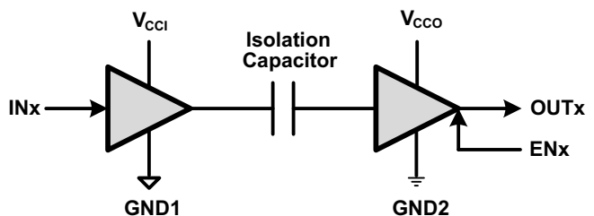
Simplified Schematic
