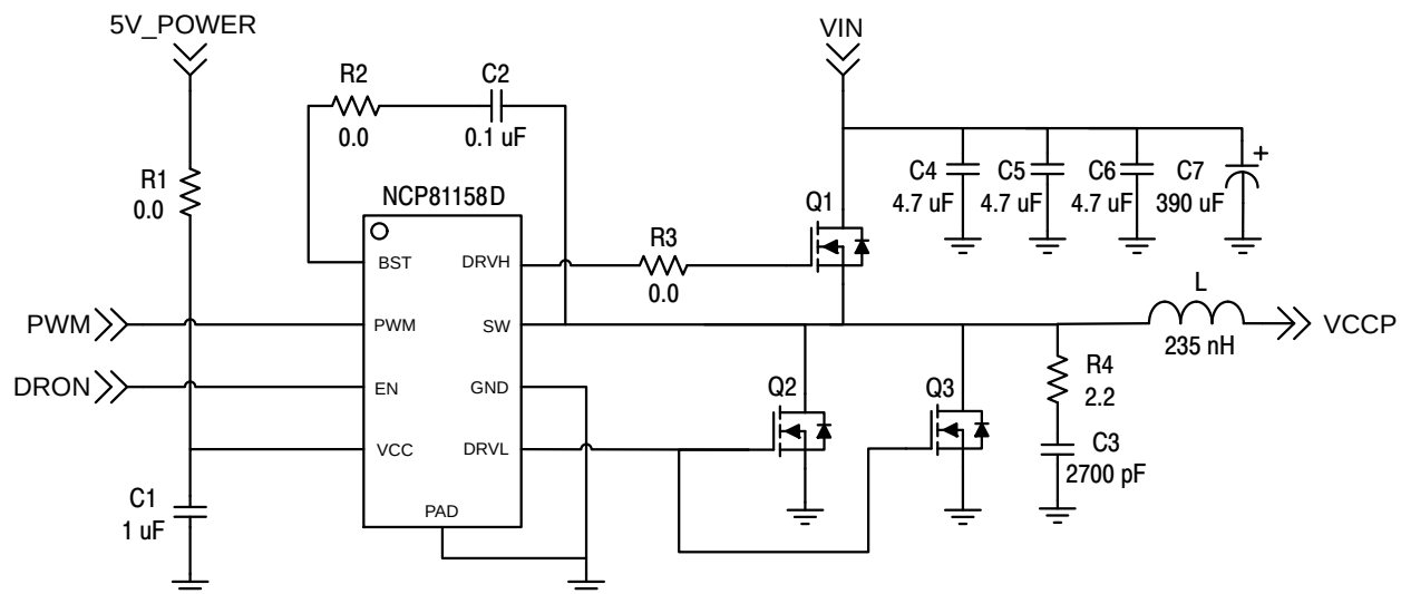
Figure 2. Application Circuit
