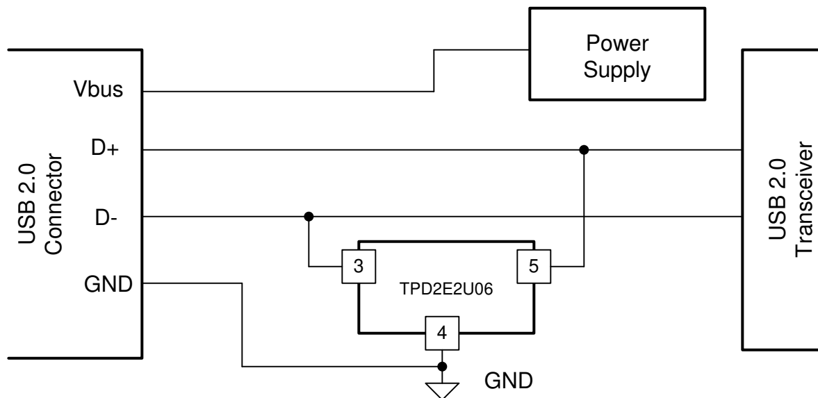
Simplified Schematic
