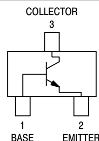
SC-75 CASE 463-01 STYLE 1
