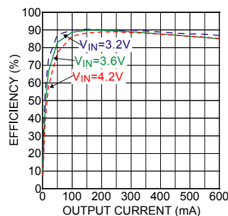
2.5Vout Efficiency
