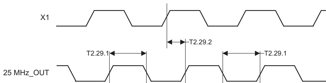
Figure 4-30. 25MHz_OUT Timing
