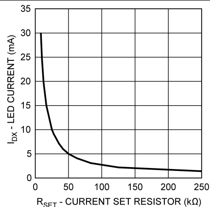
Figure 7. LED Current vs R SET
