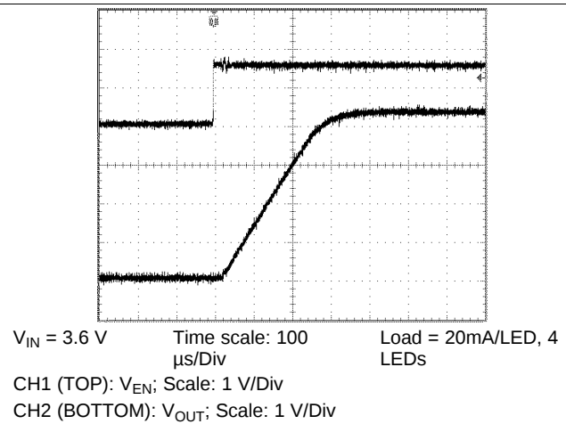
Figure 4. Start-Up Response
