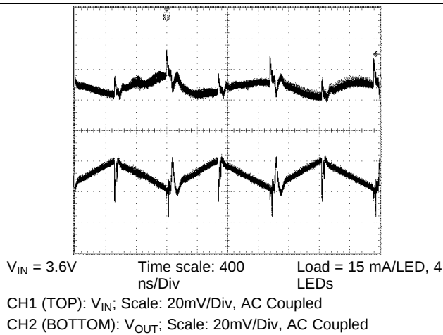
Figure 3. Input and Output Voltage Ripple
