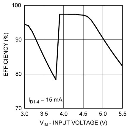
Figure 6. Converter Efficiency vs Input Voltage
