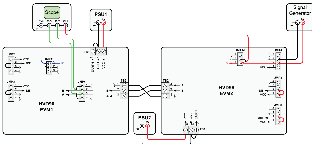
Figure 10. EVM Configurations: Left as Receiver EVM, Right as Transmitter EVM
