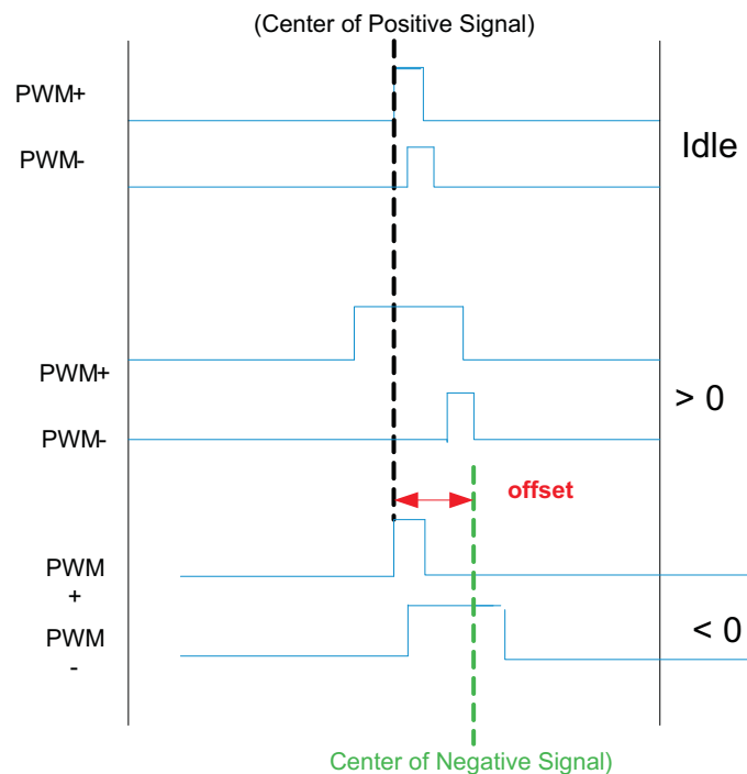
Figure 22. Ternary Modulation
