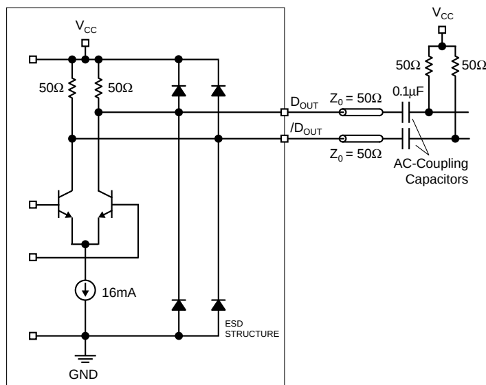
Figure 3. Output Structure
