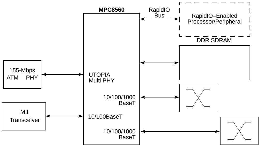
Figure 16. ATM Protocol Converter Configuration
