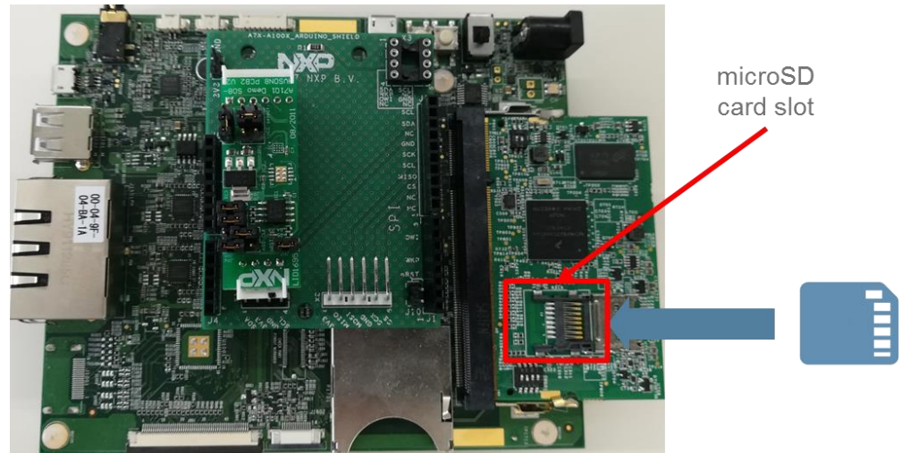
Fig 15. Insert microSD card with the pre-compiled Linux image in the microSD card slot
