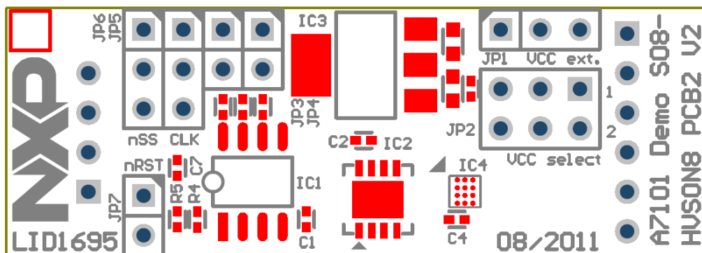
Fig 4. OM3710/A71CHPCB board silkscreen
