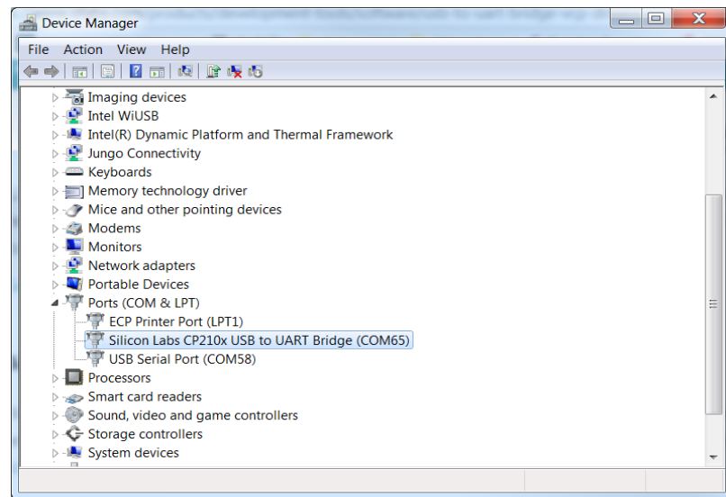
Fig 12. Device manager
