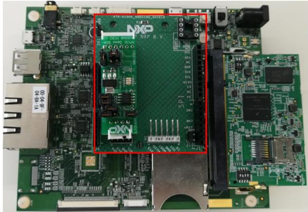
Fig 9. OM3710/A71CHARD mounted on the i.MXUltraLite board (MCIMXUL-EVKB).
